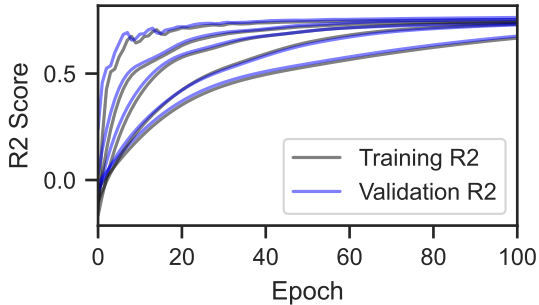
R2 Score History
