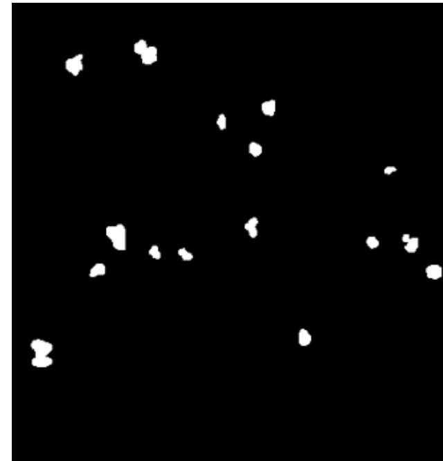
Ground truth
