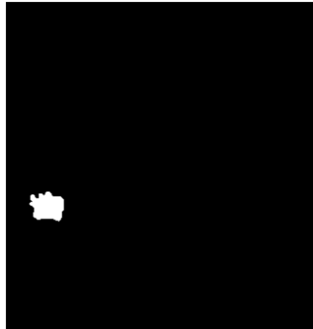
Ground truth
