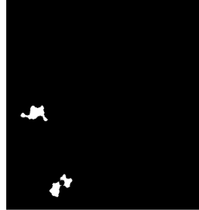
Final mask
