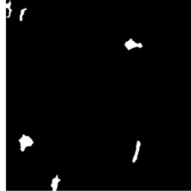
Final mask
