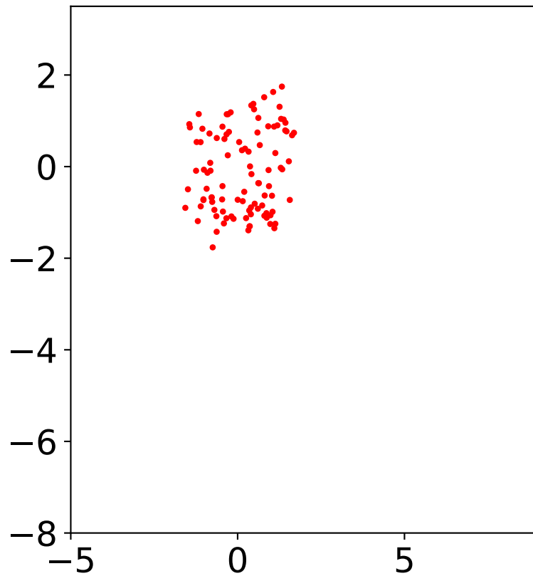
P-ZOD-MC
