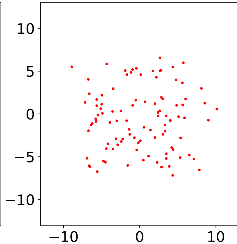
P-ZOD-MC
