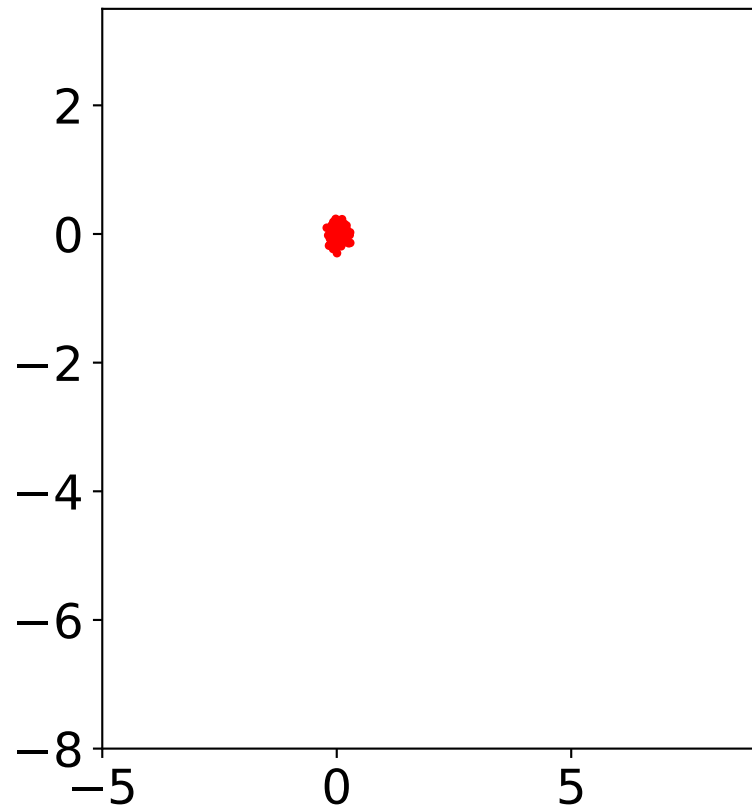
ZOD-MC
