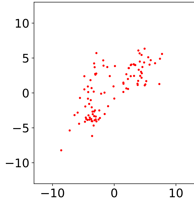
Ground Truth
