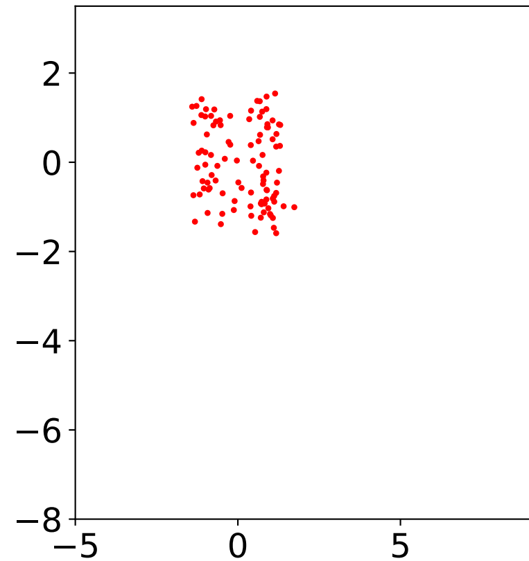
Ground Truth
