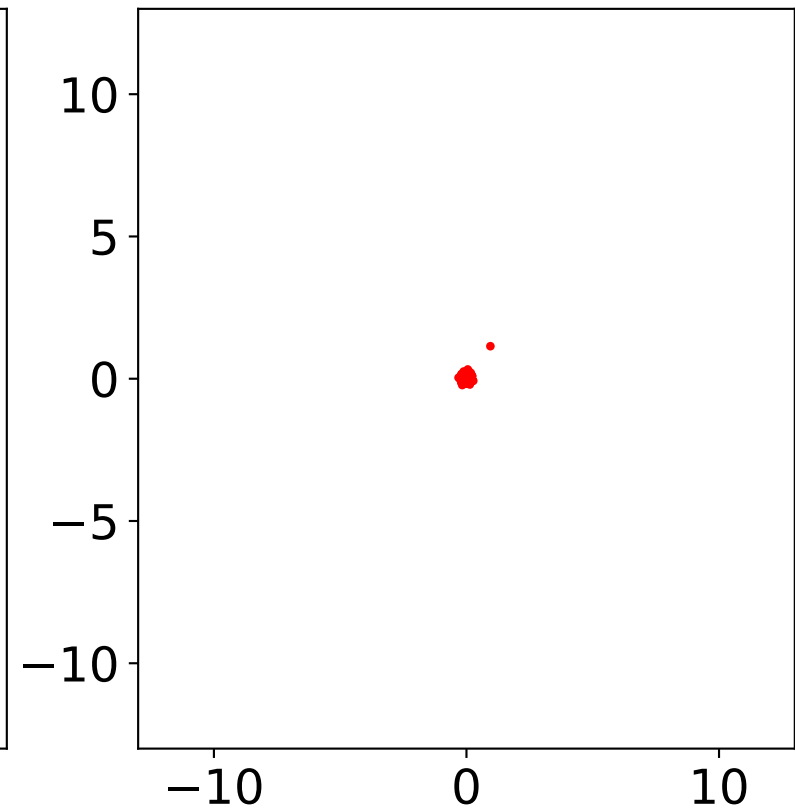
ZOD-MC
