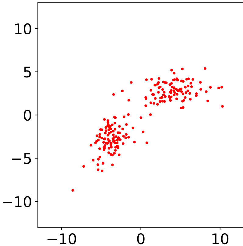
Ground Truth
