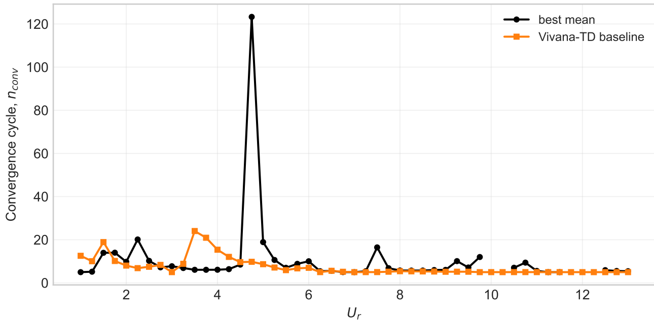
Persistent rolling-std convergence cycle
