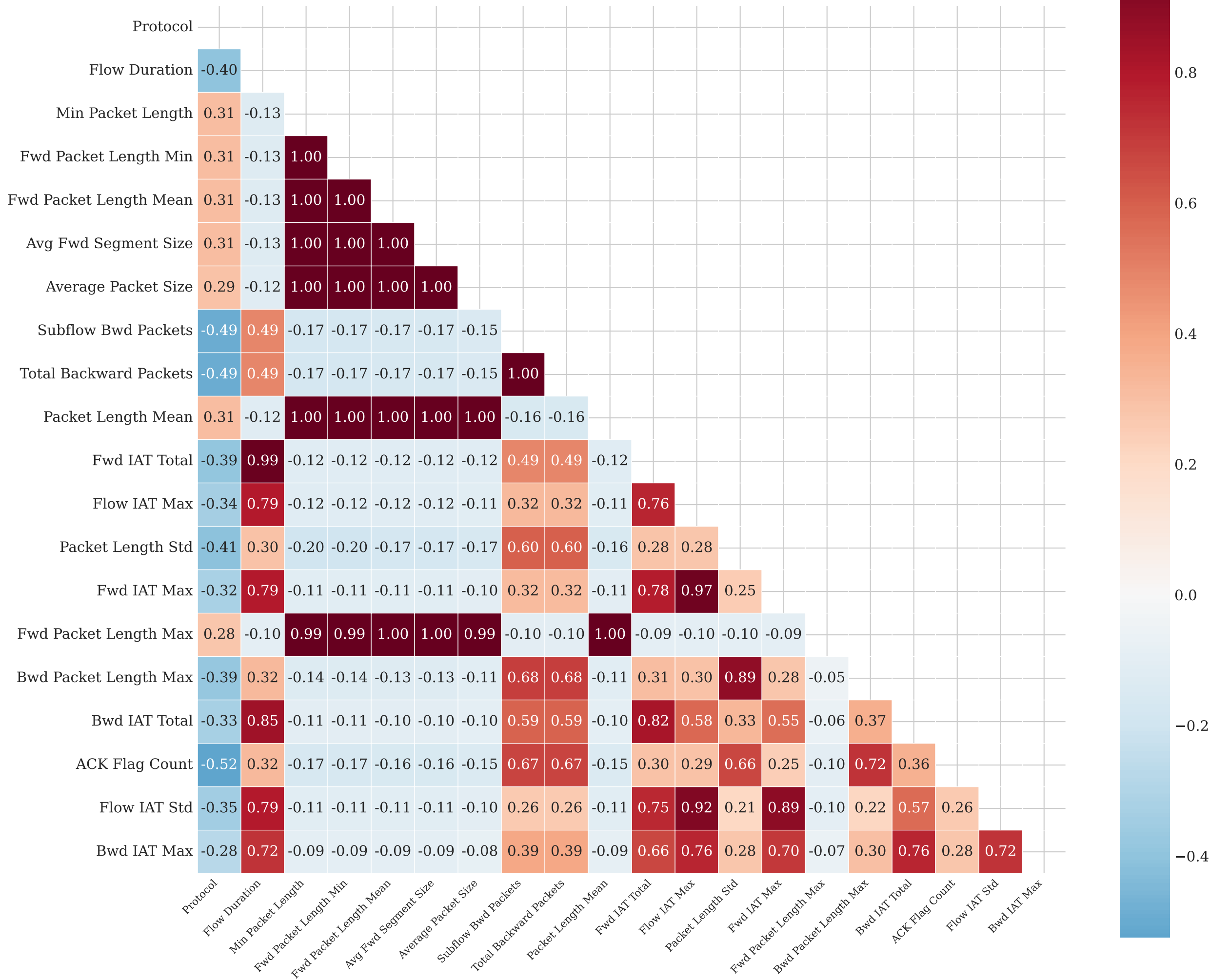
Figure 3.1: Correlation Heatmap of Top Twenty Selected Features
