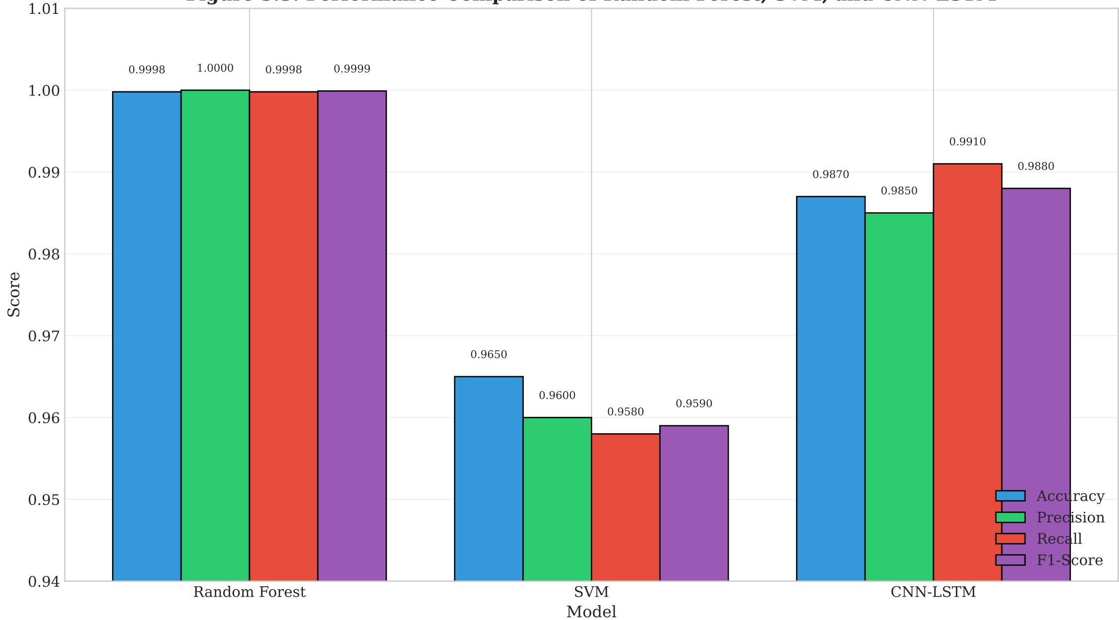
Figure 3.3: Performance Comparison of Random Forest, SVM, and CNN-LSTM
