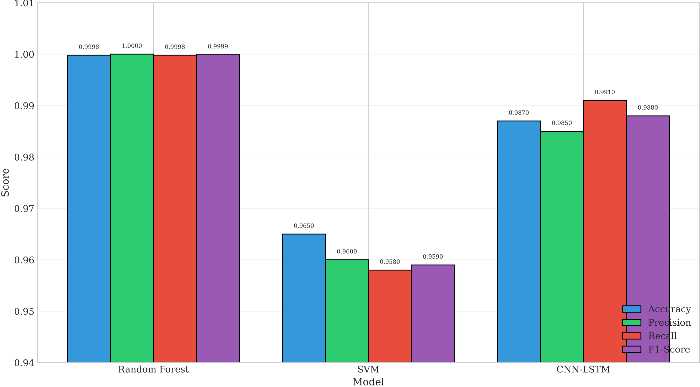
Figure 4.3: Performance Comparison of Random Forest, SVM, and CNN-LSTM Models
