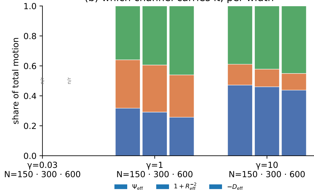
(b) which channel carries it, per width
