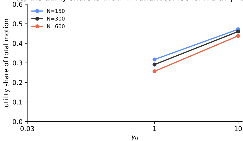
(c) the utility share is width-invariant (0.438-0.472 at \gamma=10 )
