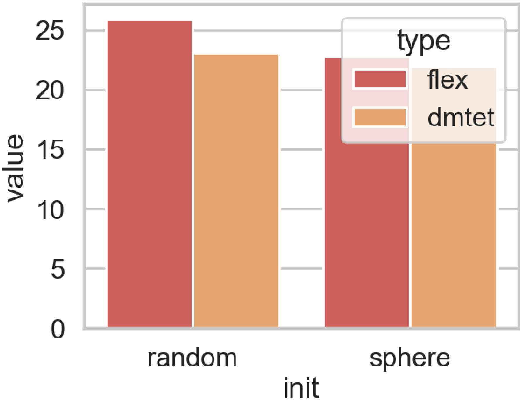
Figure 3: PSNR at Test time (ShapeNet)
