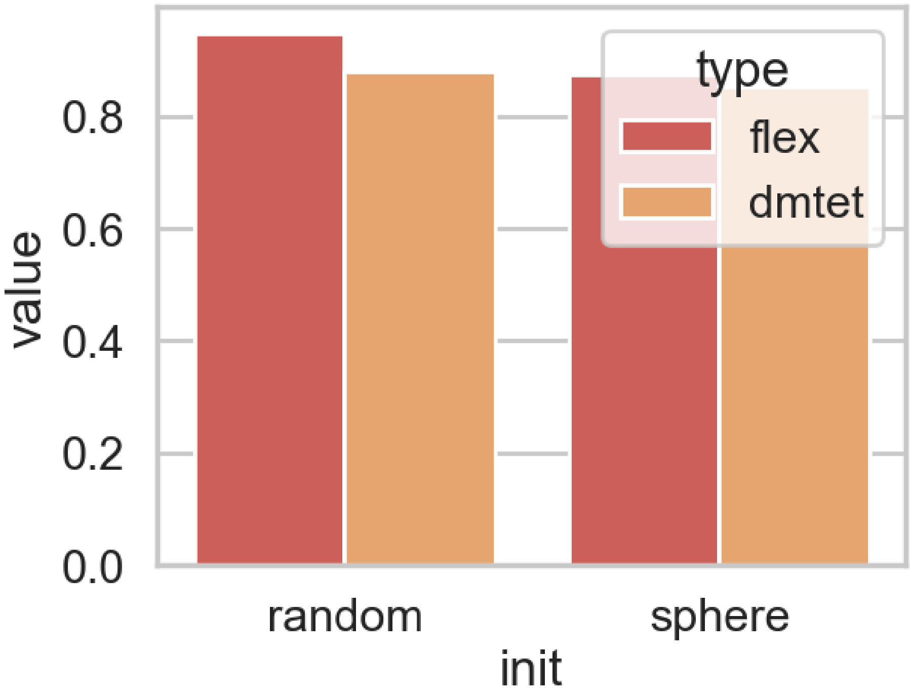
Figure 1: IoU at Test time (ShapeNet)
