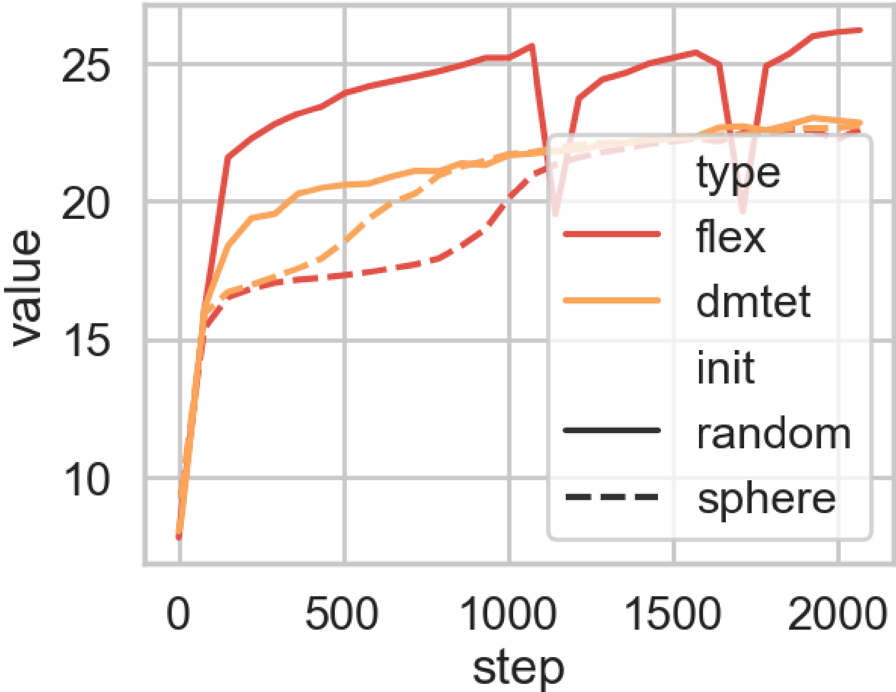
Figure 4: PSNR on Validation Set during Training
