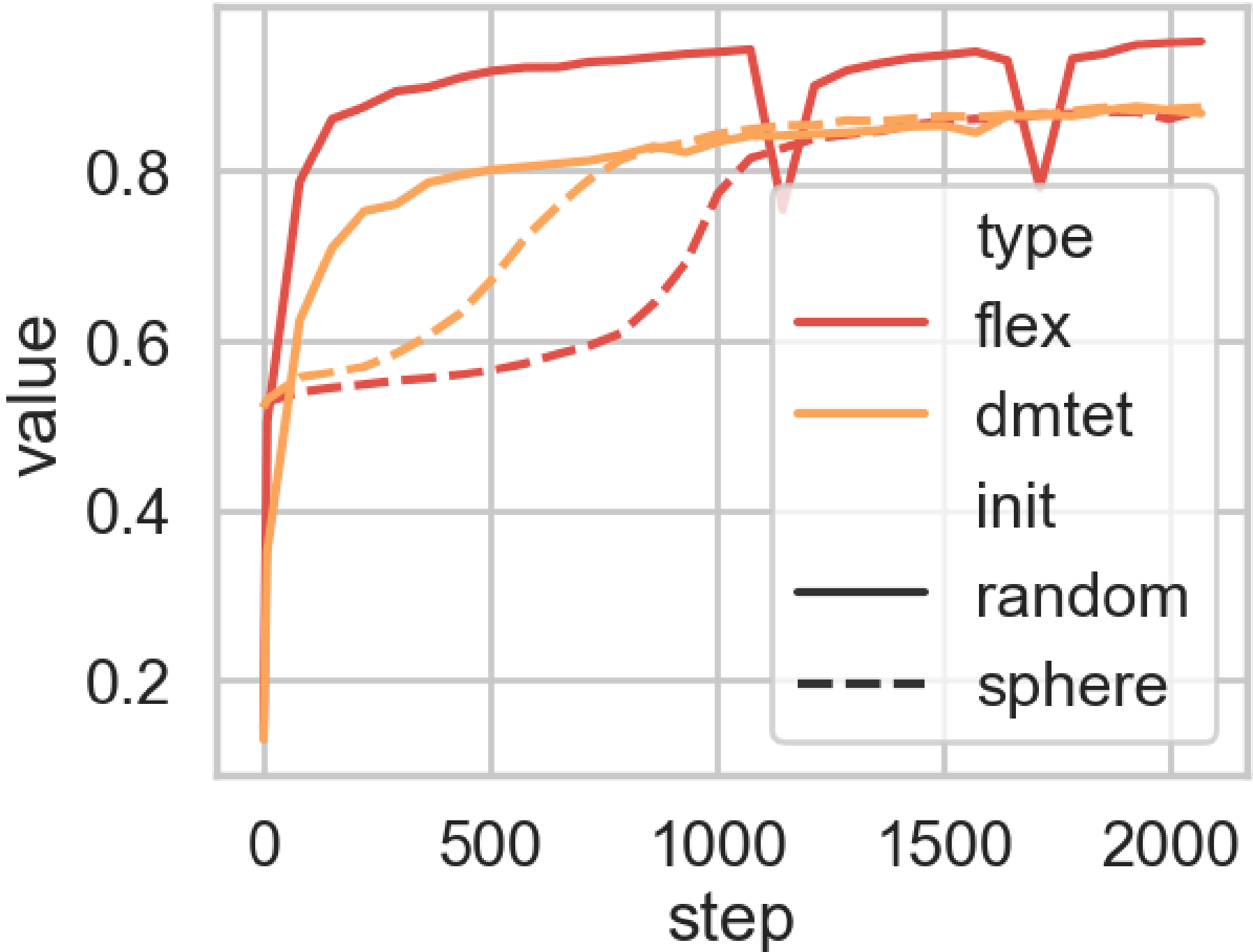
Figure 2: IoU on Validation Set during Training
