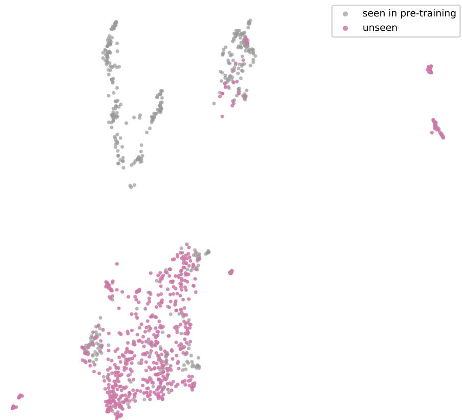
(c) Coloured by pre-training exposure
