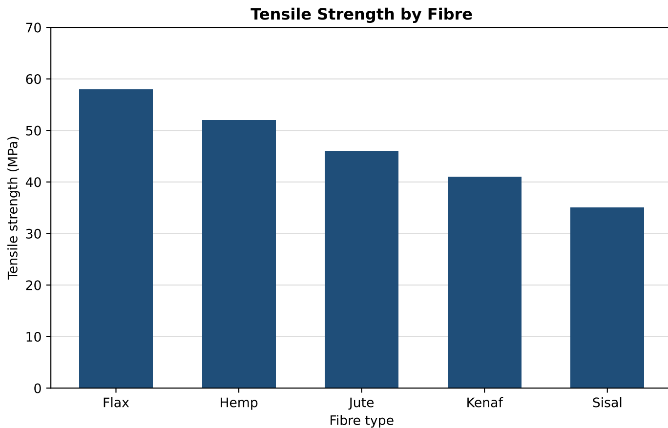
Figure 2. Ultimate tensile strength of composites reinforced with different natural fibres. Error bars omitted for clarity.
