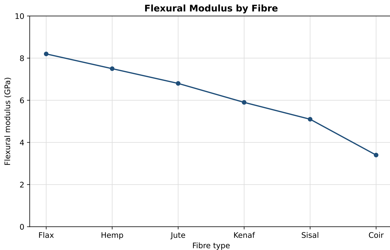
Figure 3. Flexural modulus across fibre types, plotted as a line to emphasise the monotonic trend (the x axis is categorical, not numeric).
