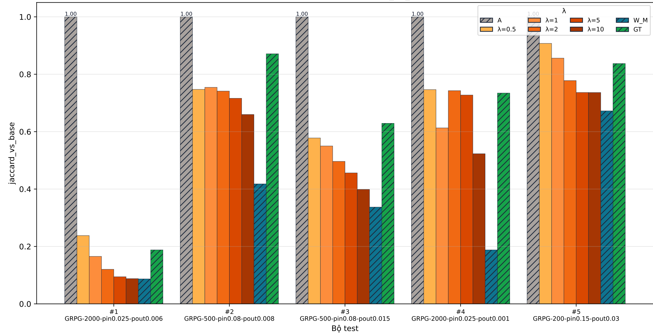
[GRPG] stability · jaccard_vs_base
