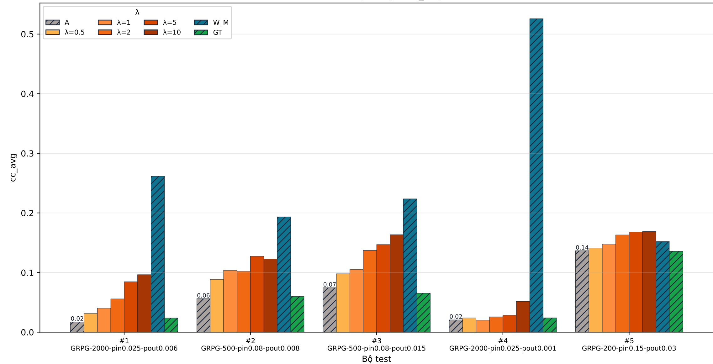
[GRPG] quality · cc_avg
