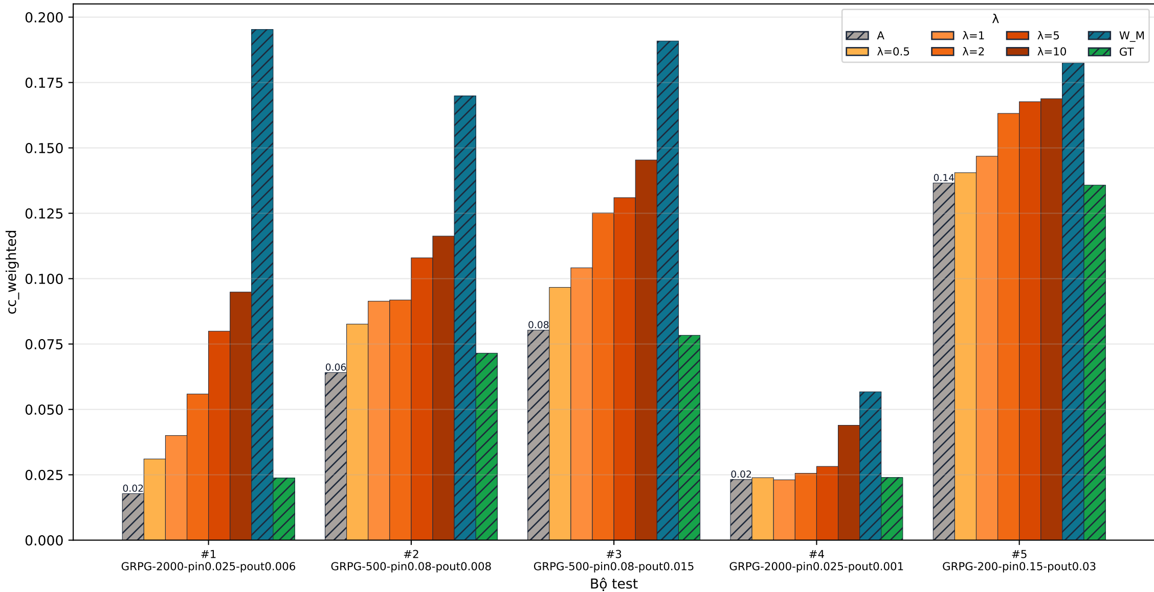
[GRPG] quality · cc_weighted
