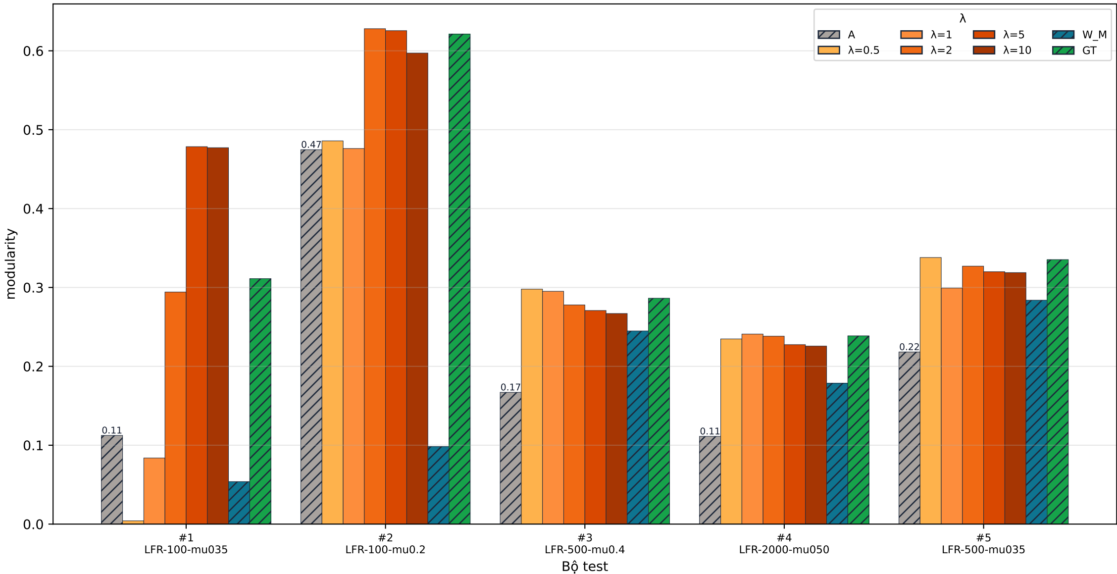
[LFR] quality · modularity
