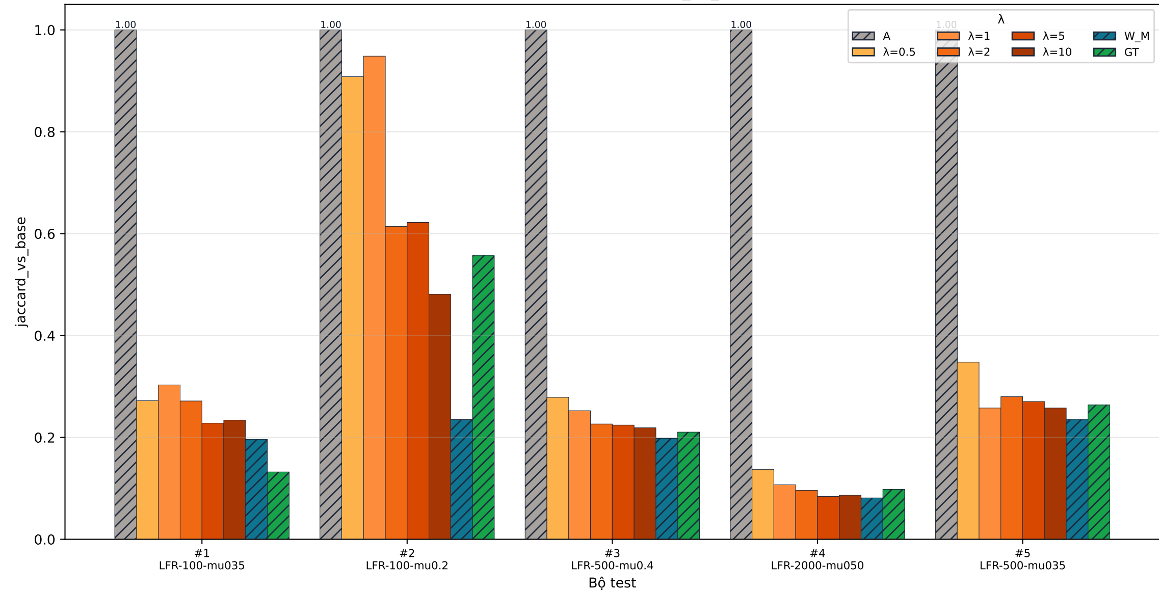
[LFR] stability · jaccard_vs_base
