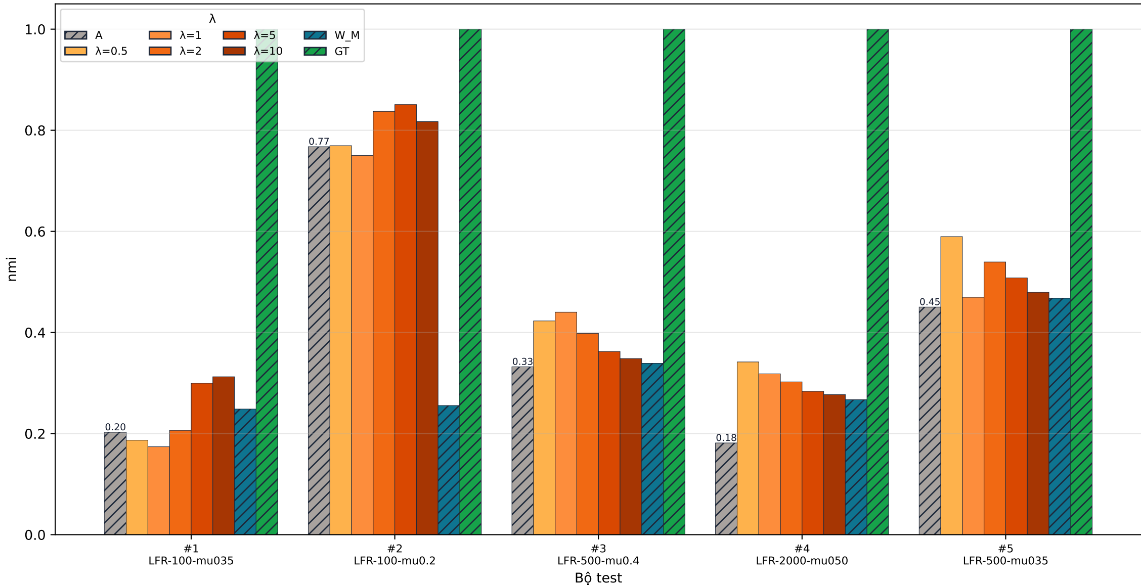
[LFR] compare_to_GT · nmi
