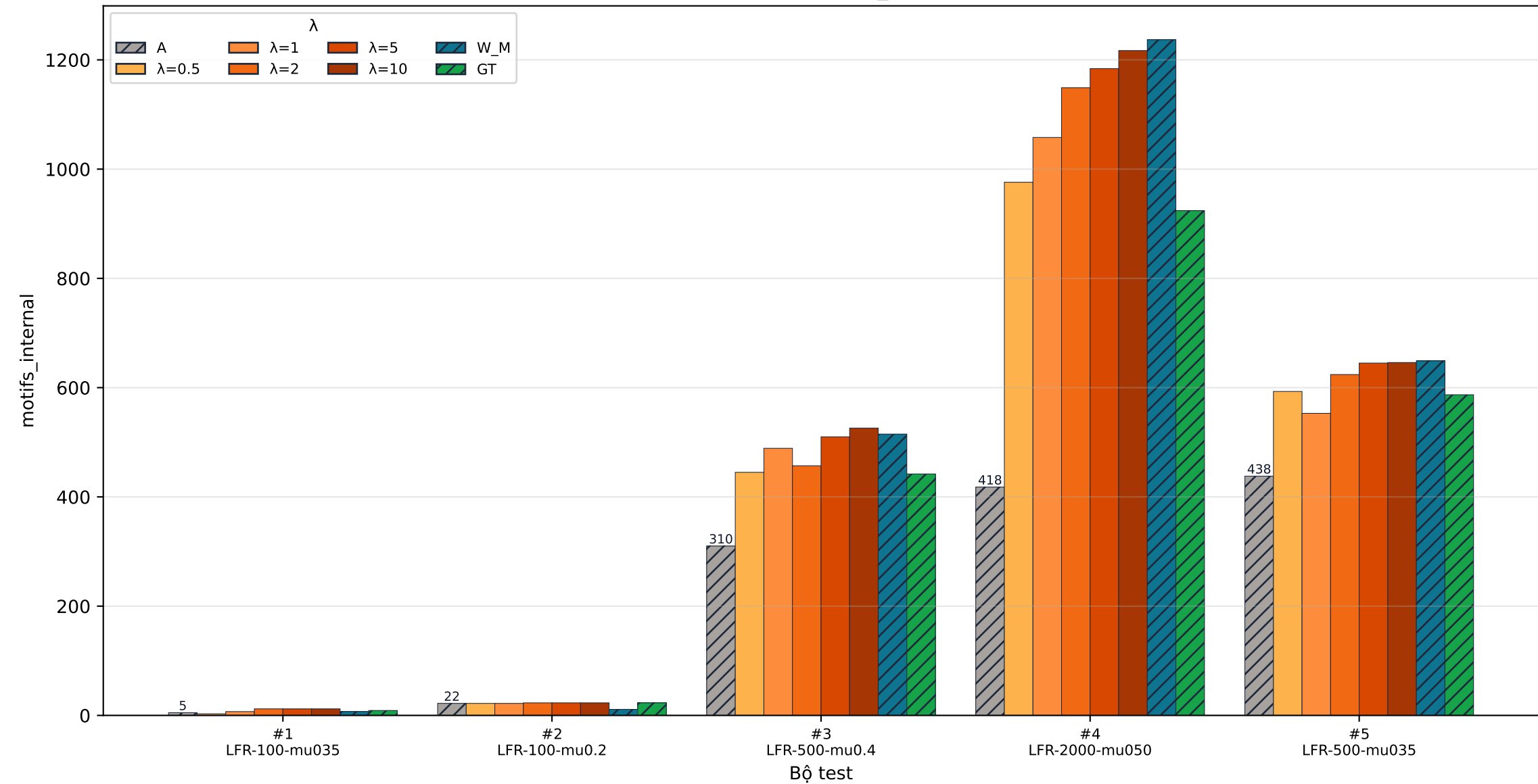
[LFR] cut · motifs_internal
