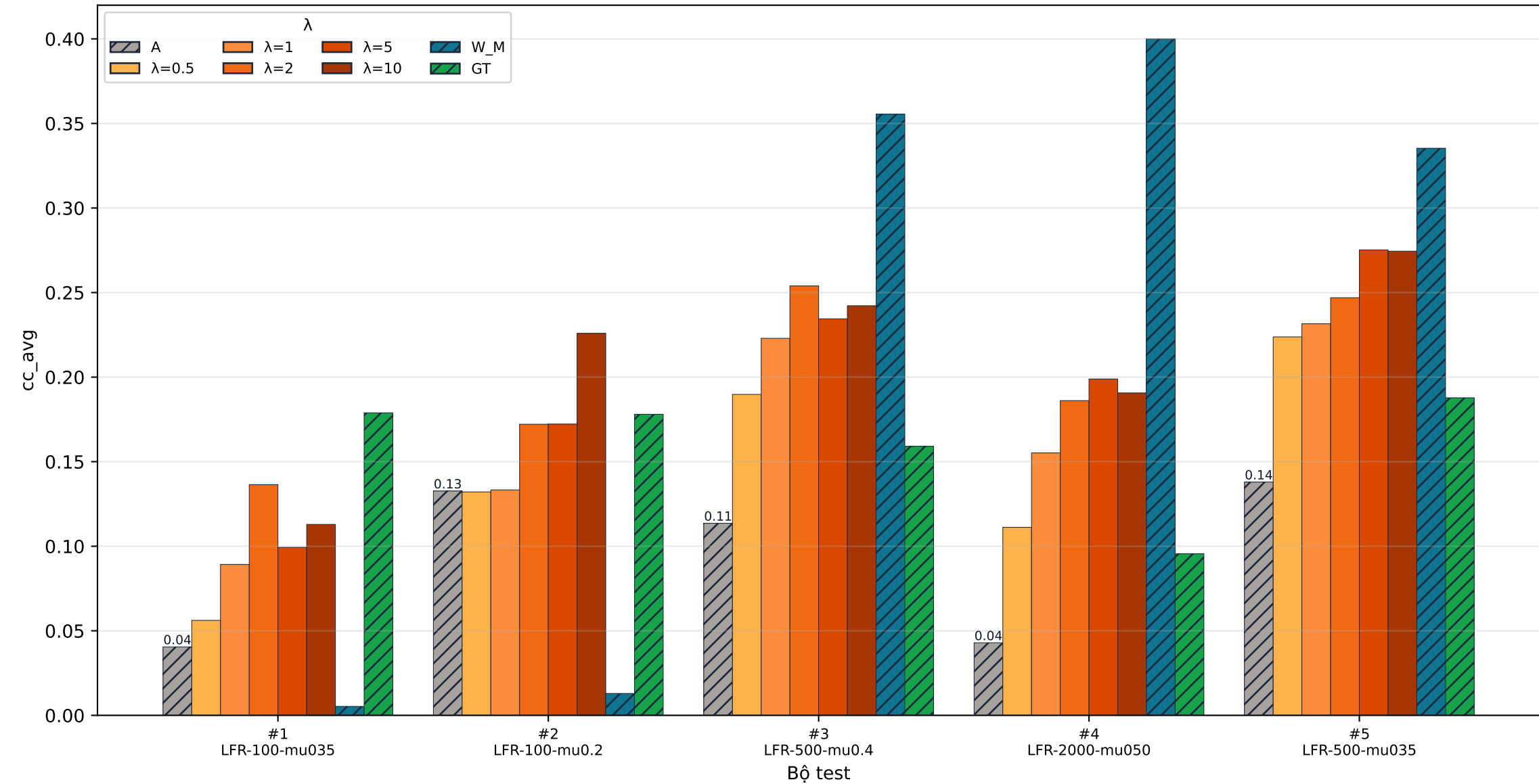
[LFR] quality · cc_avg
