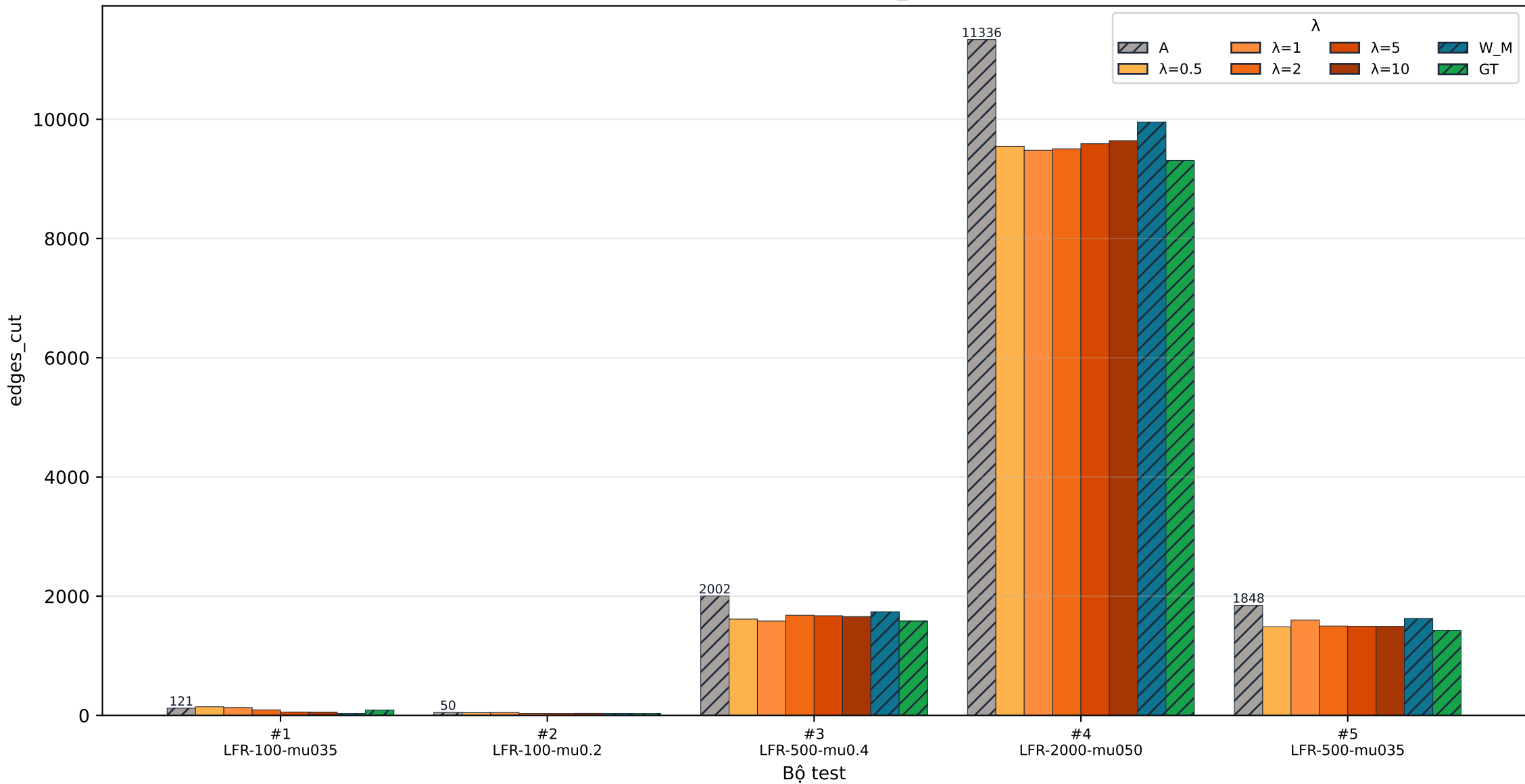
[LFR] cut · edges_cut
