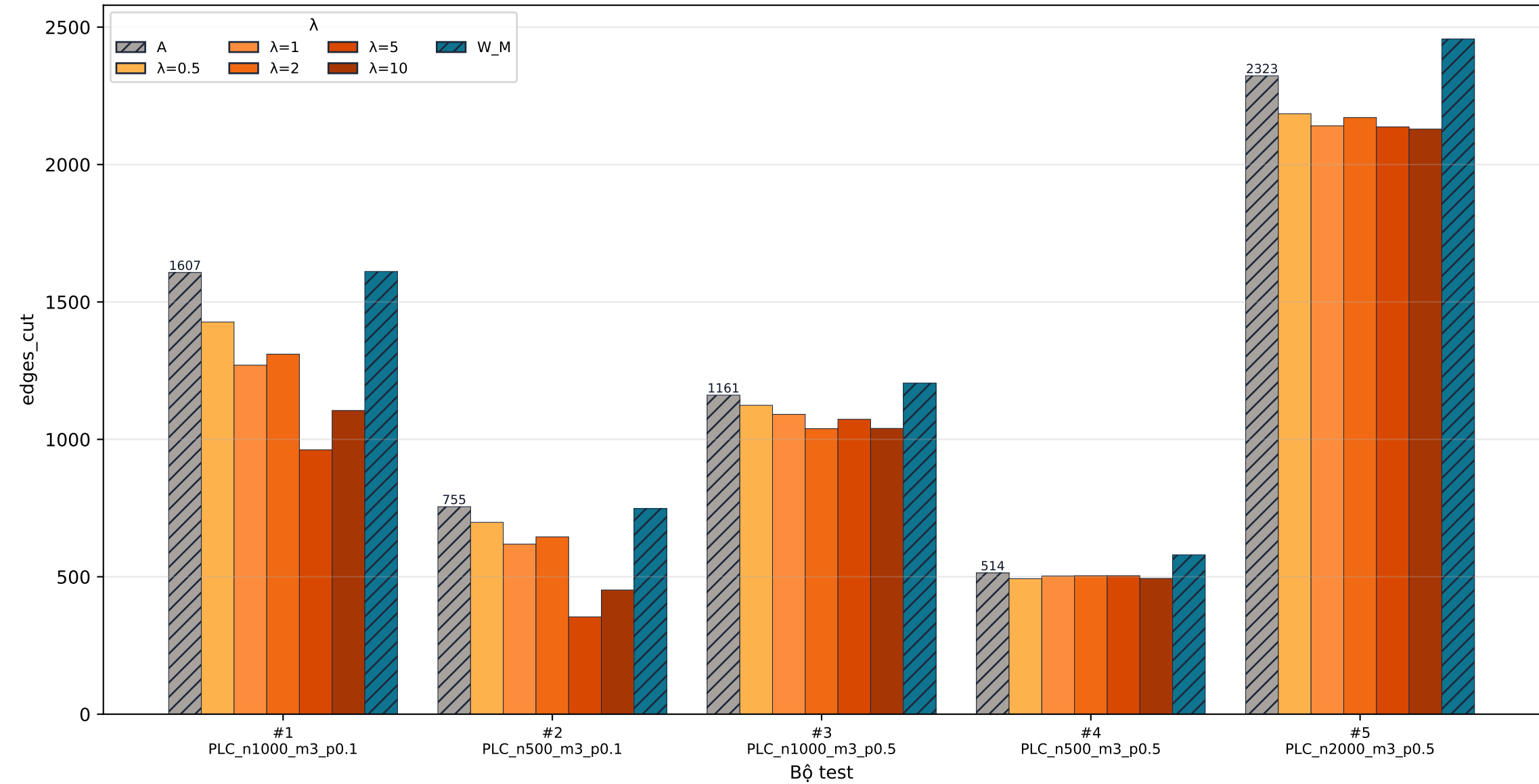
[PLC] cut · edges_cut
