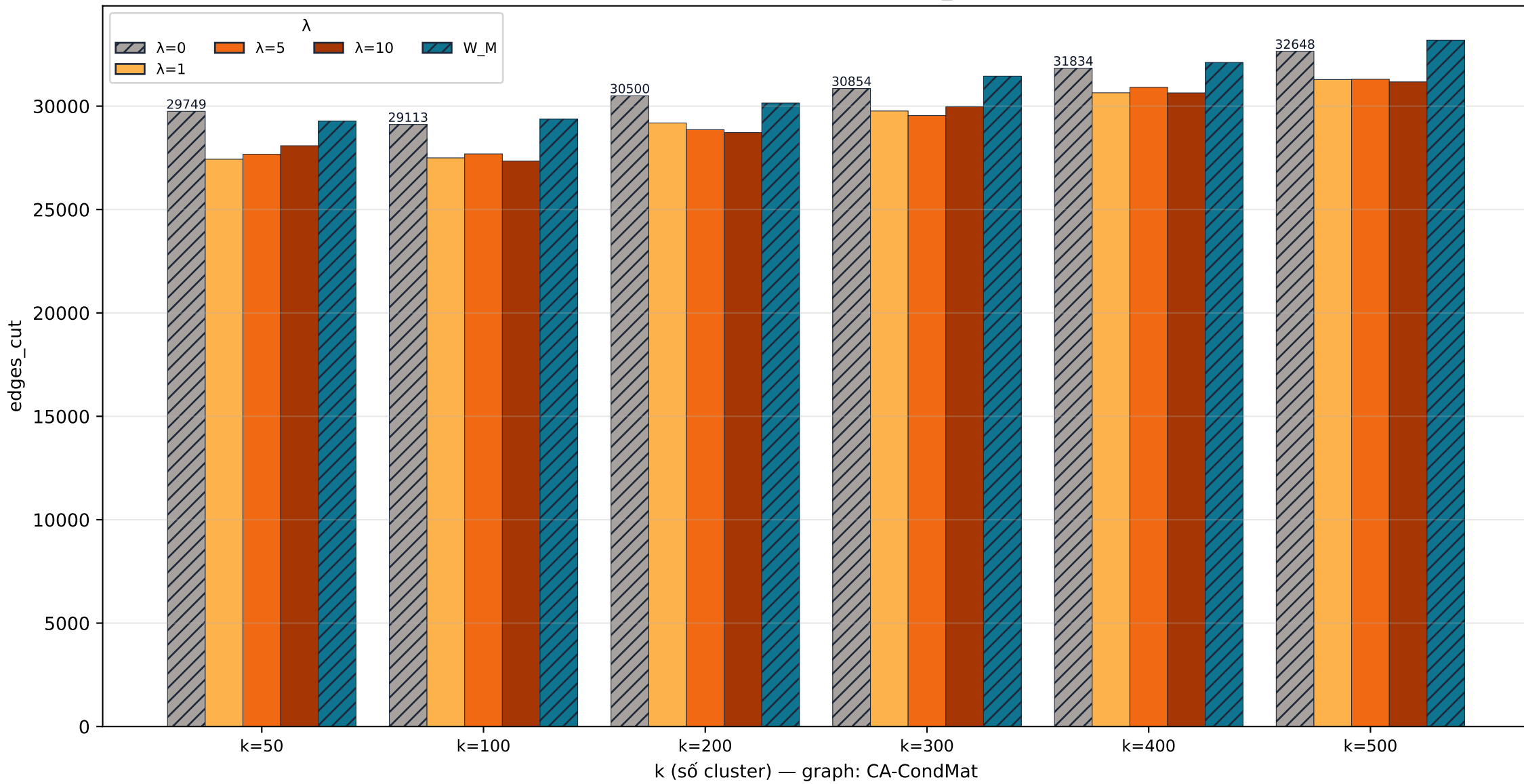
CA-CondMat cut · edges_cut
