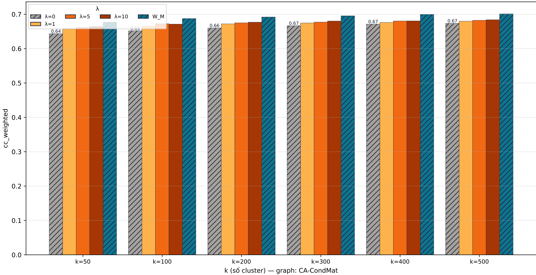
CA-CondMat quality · cc_weighted
