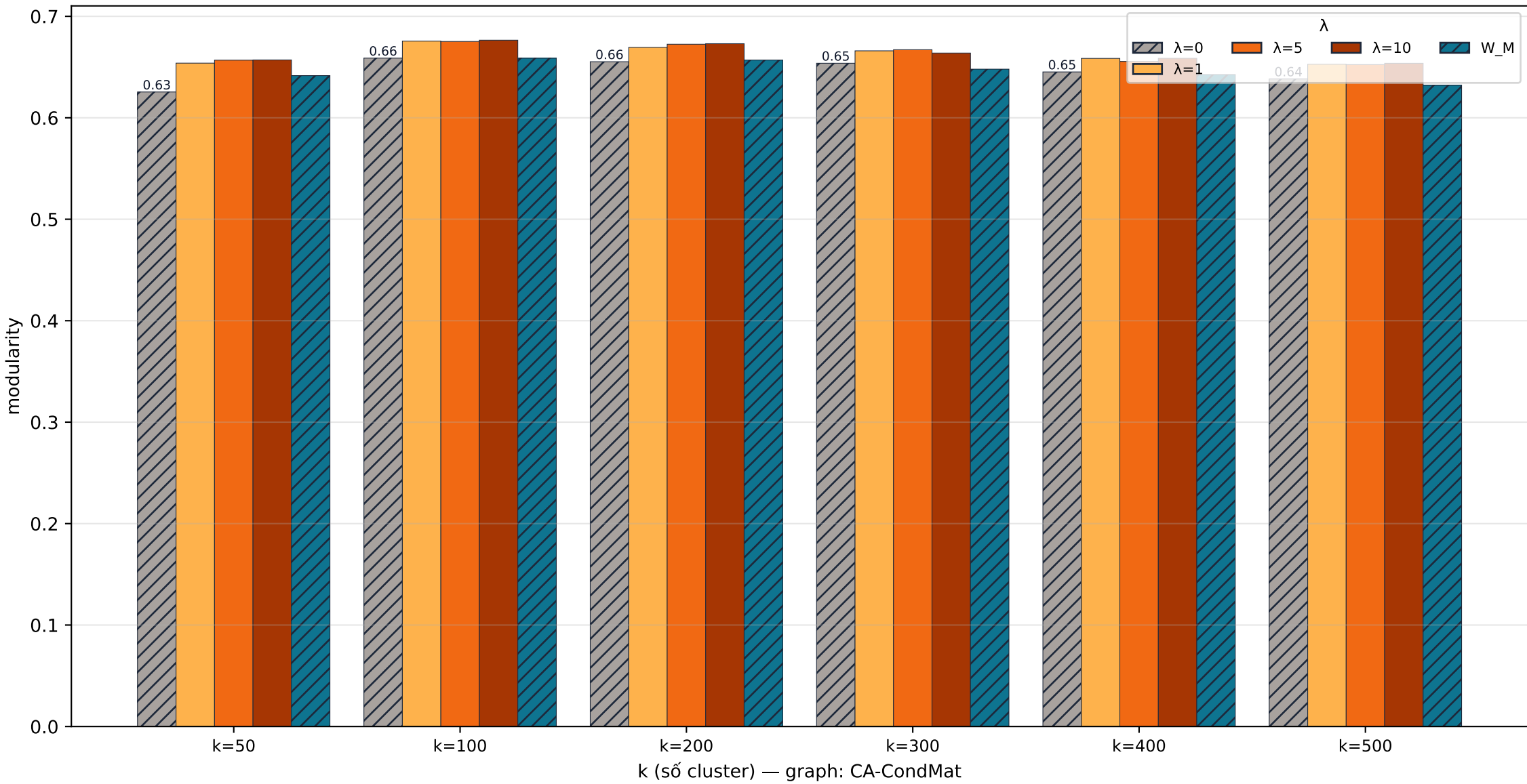
CA-CondMat quality · modularity
