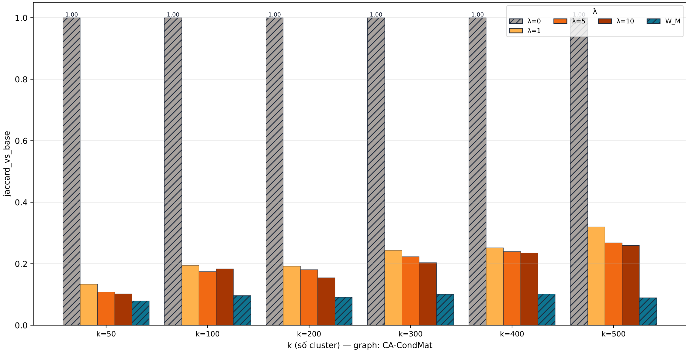
CA-CondMat stability · jaccard_vs_base
