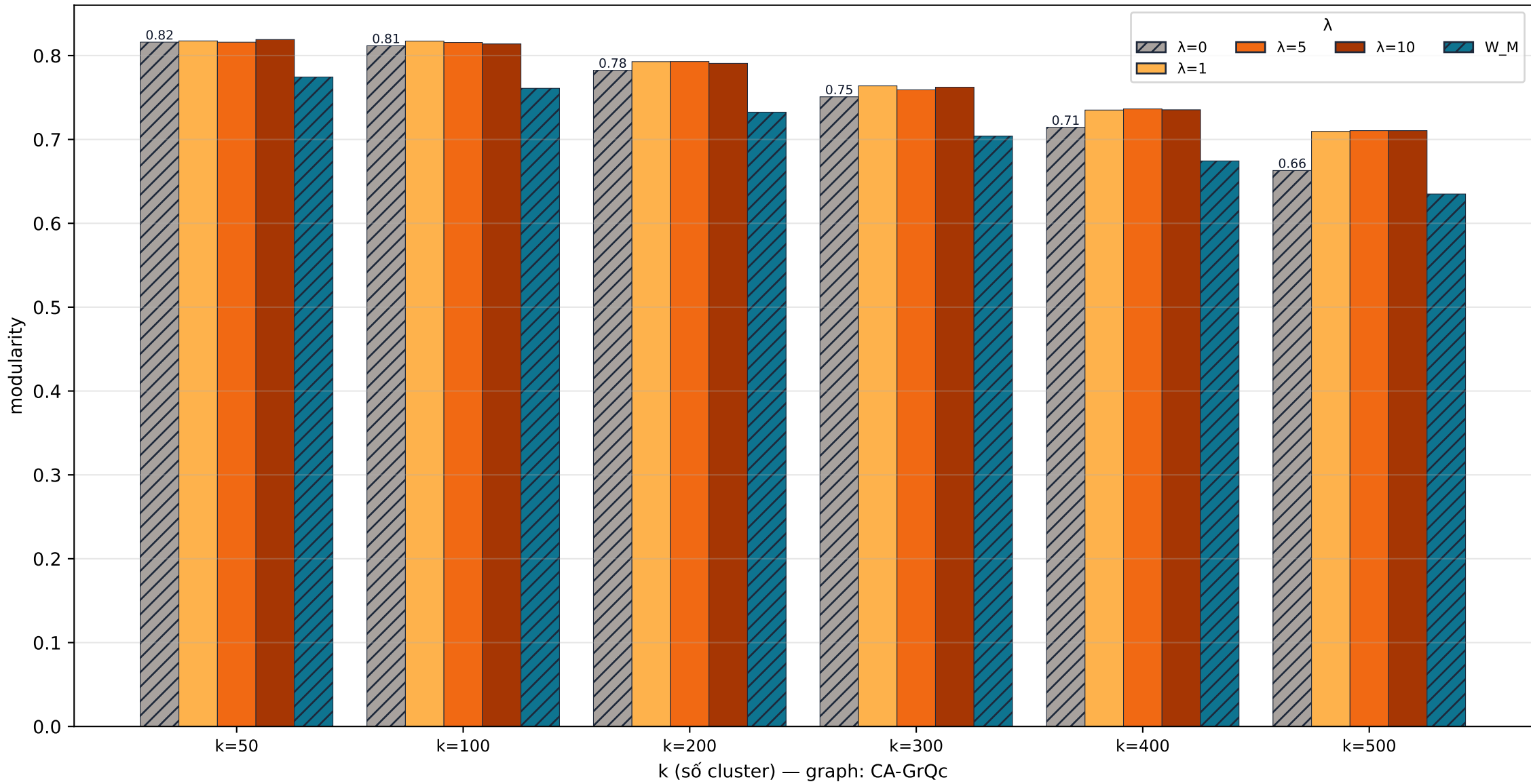
CA-GrQc quality · modularity
