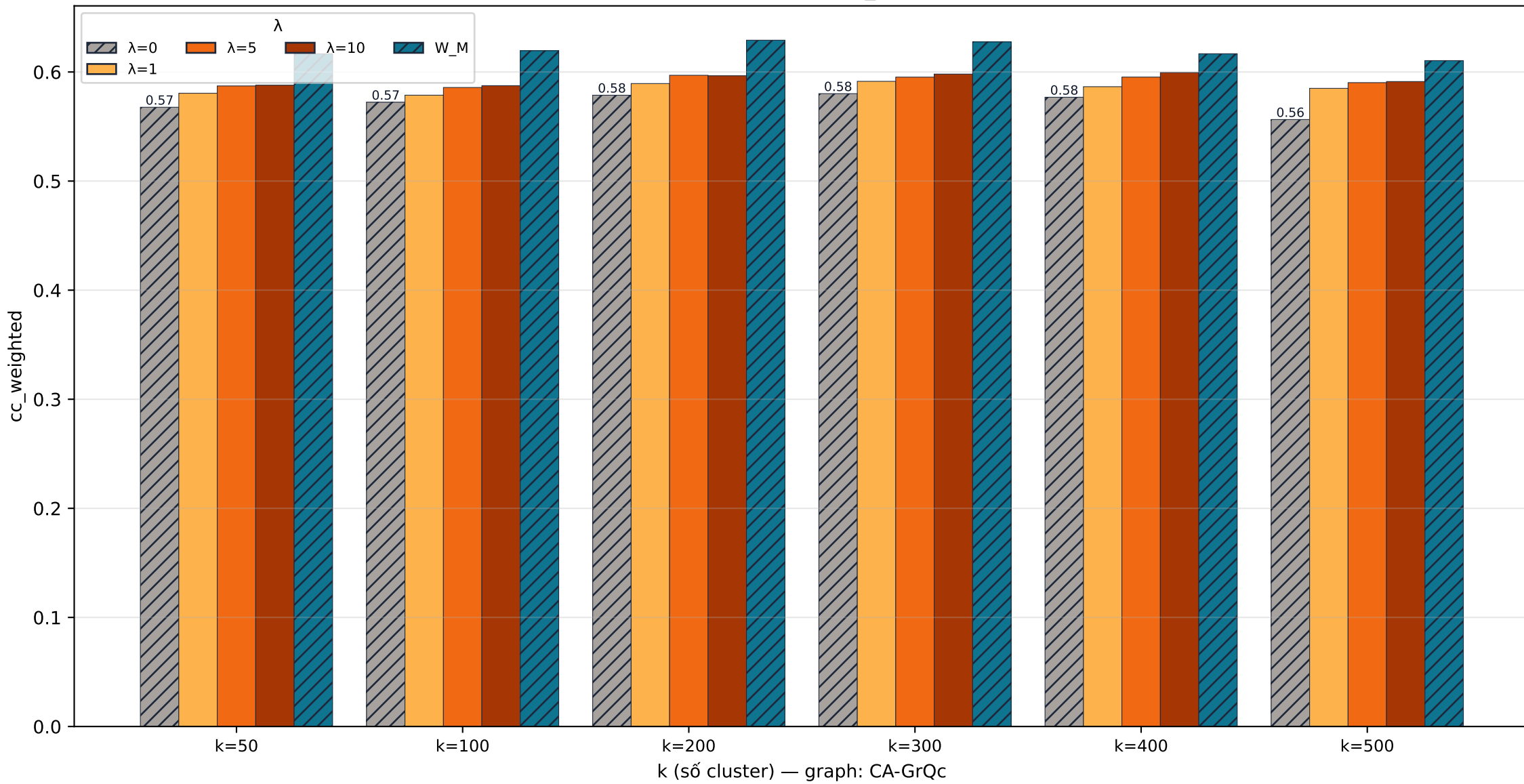
CA-GrQc quality · cc_weighted
