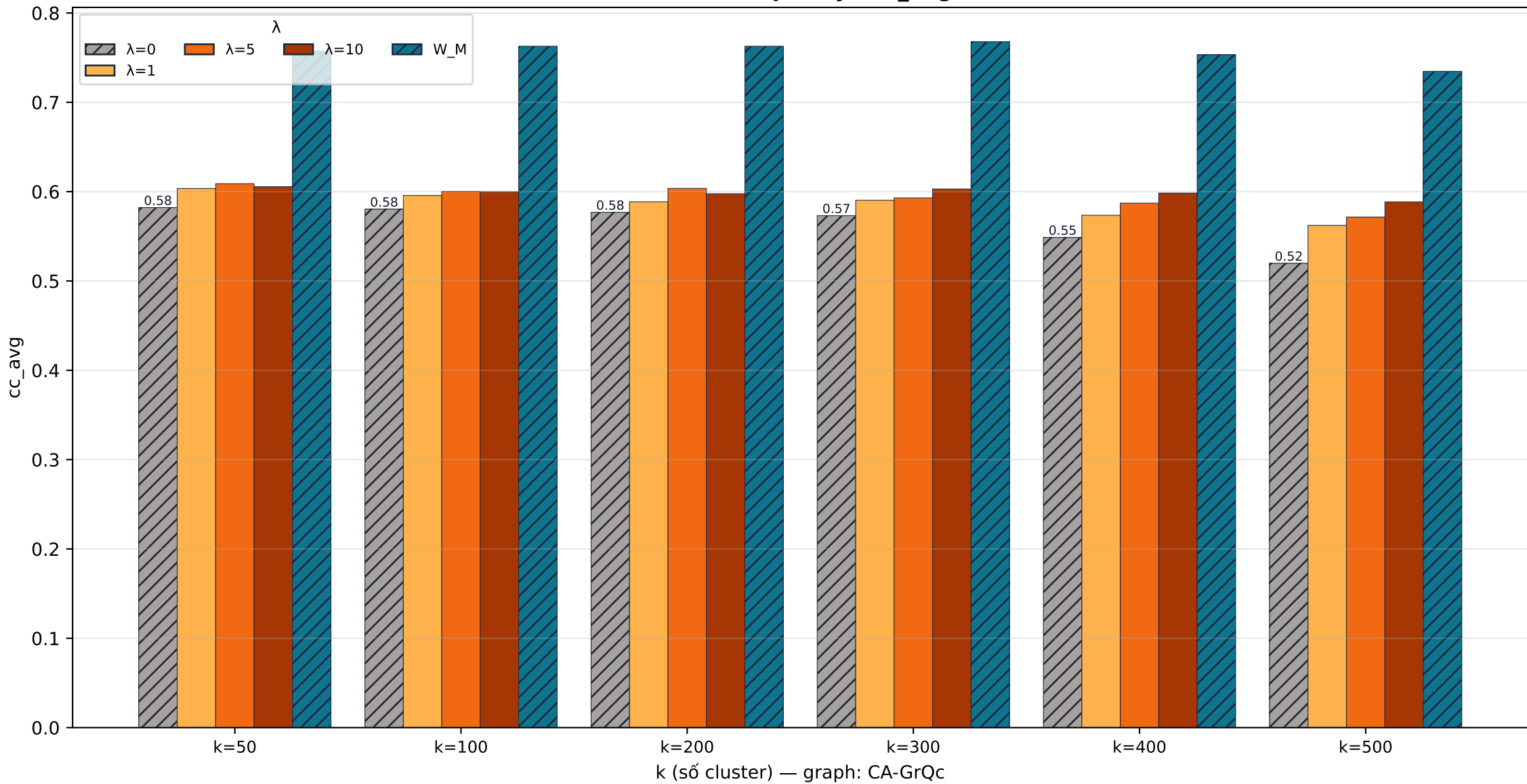
CA-GrQc quality · cc_avg
