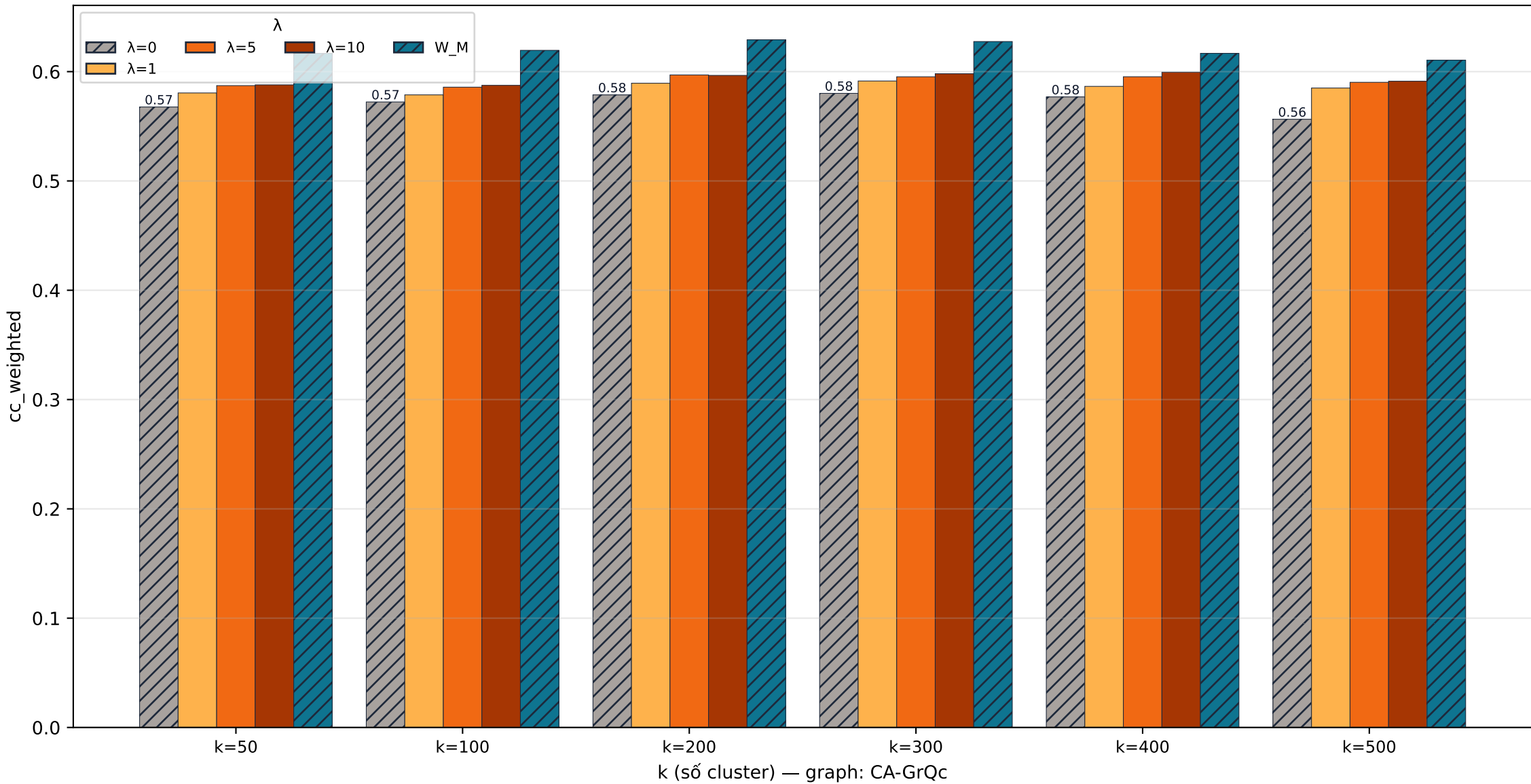
CA-GrQc quality · cc_weighted
