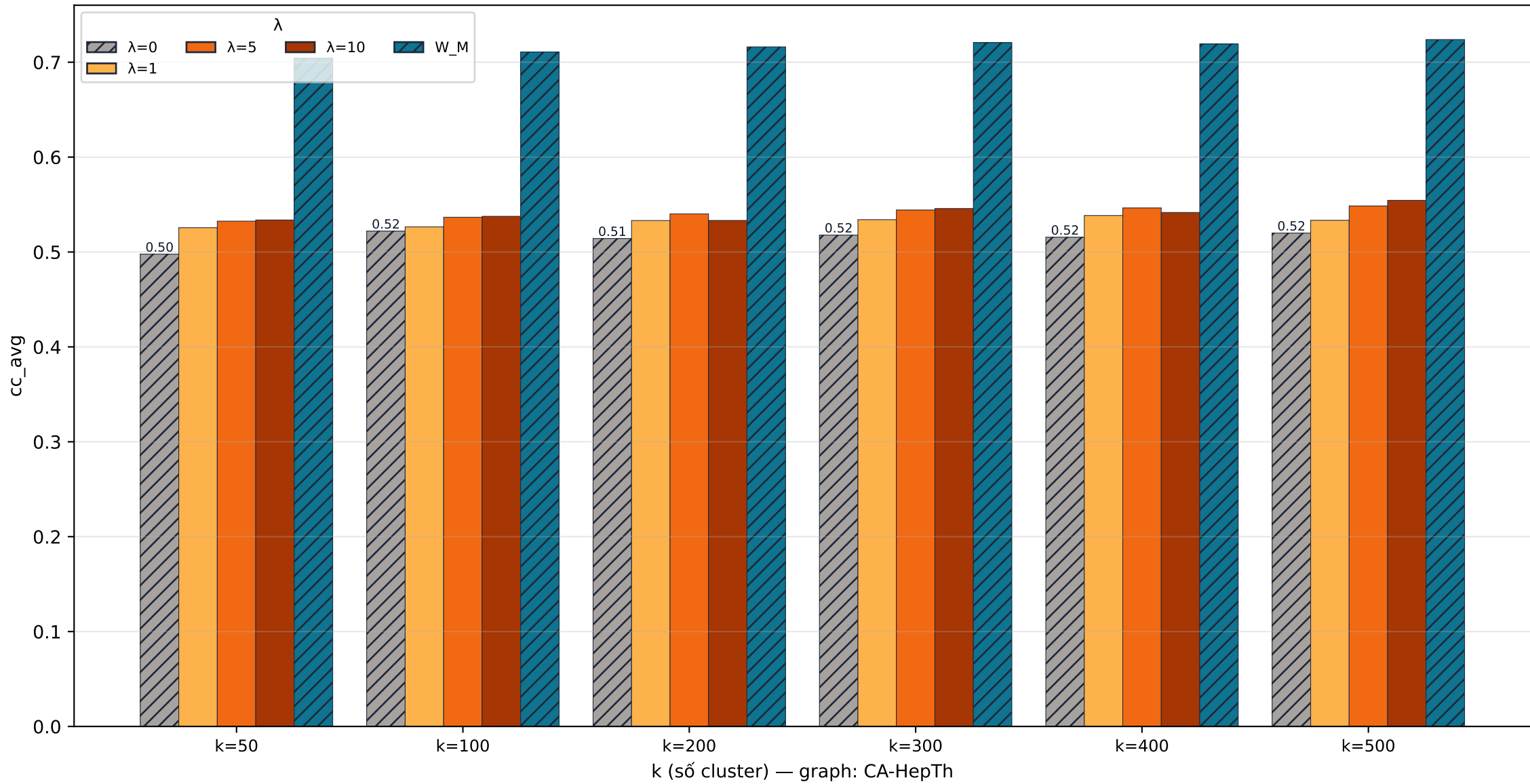
CA-HepTh quality · cc_avg
