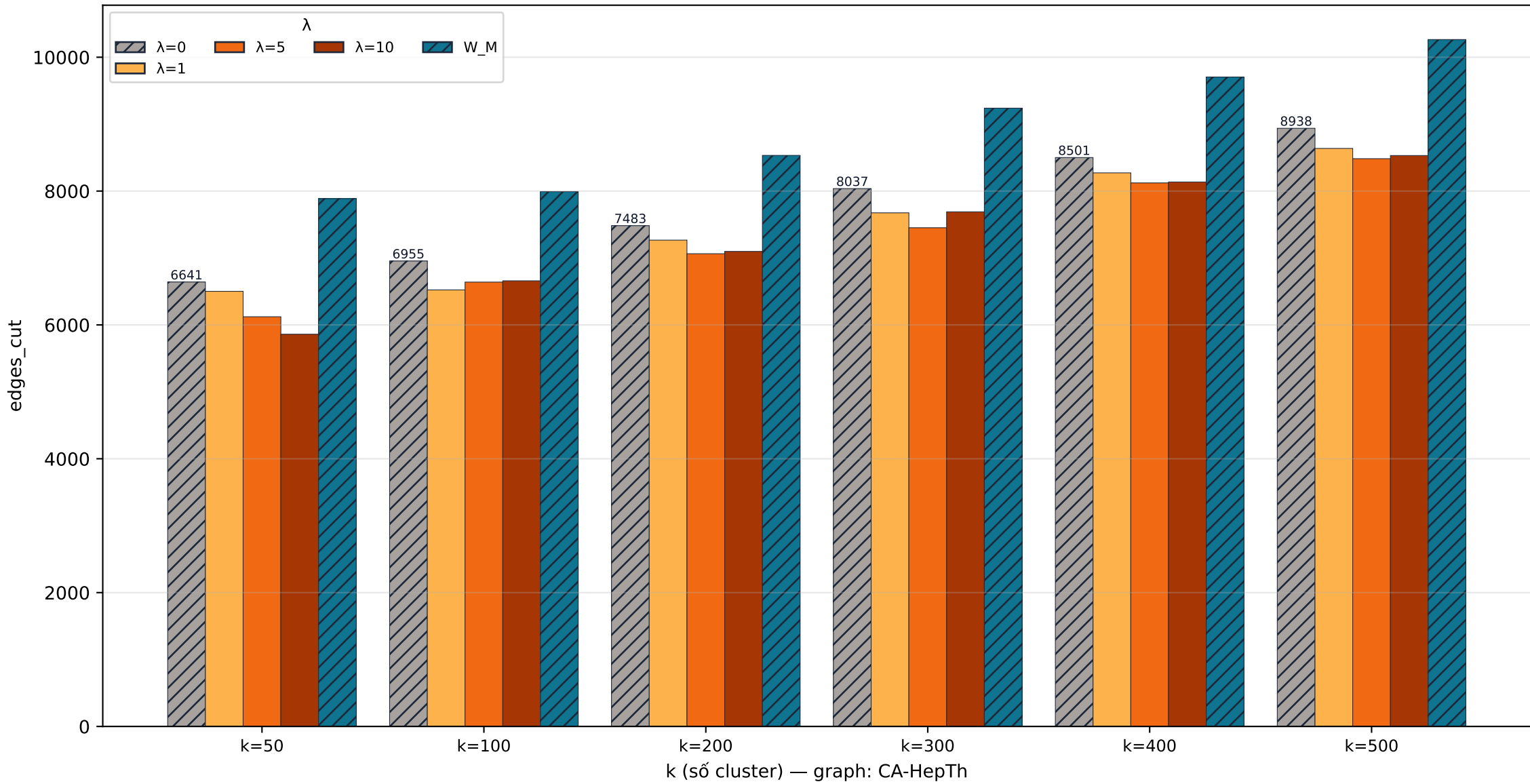
CA-HepTh cut · edges_cut
