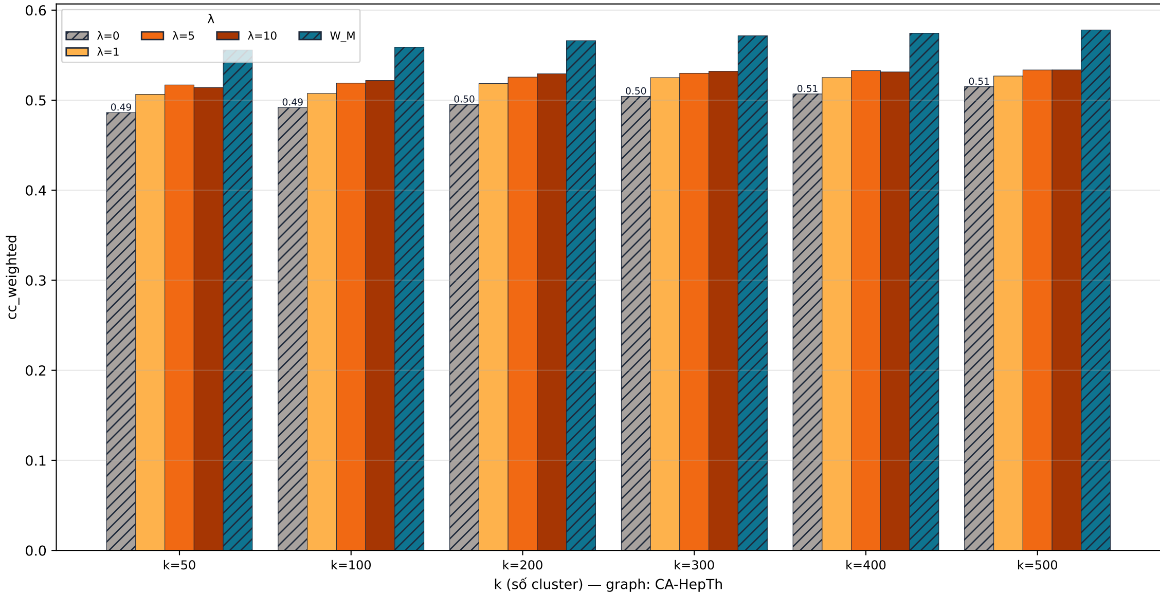
CA-HepTh quality · cc_weighted
