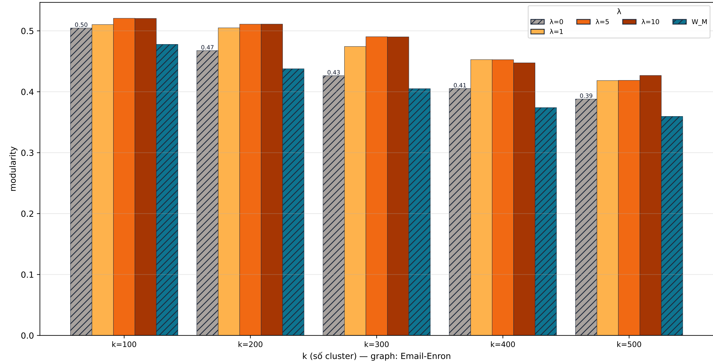
Email-Enron quality · modularity
