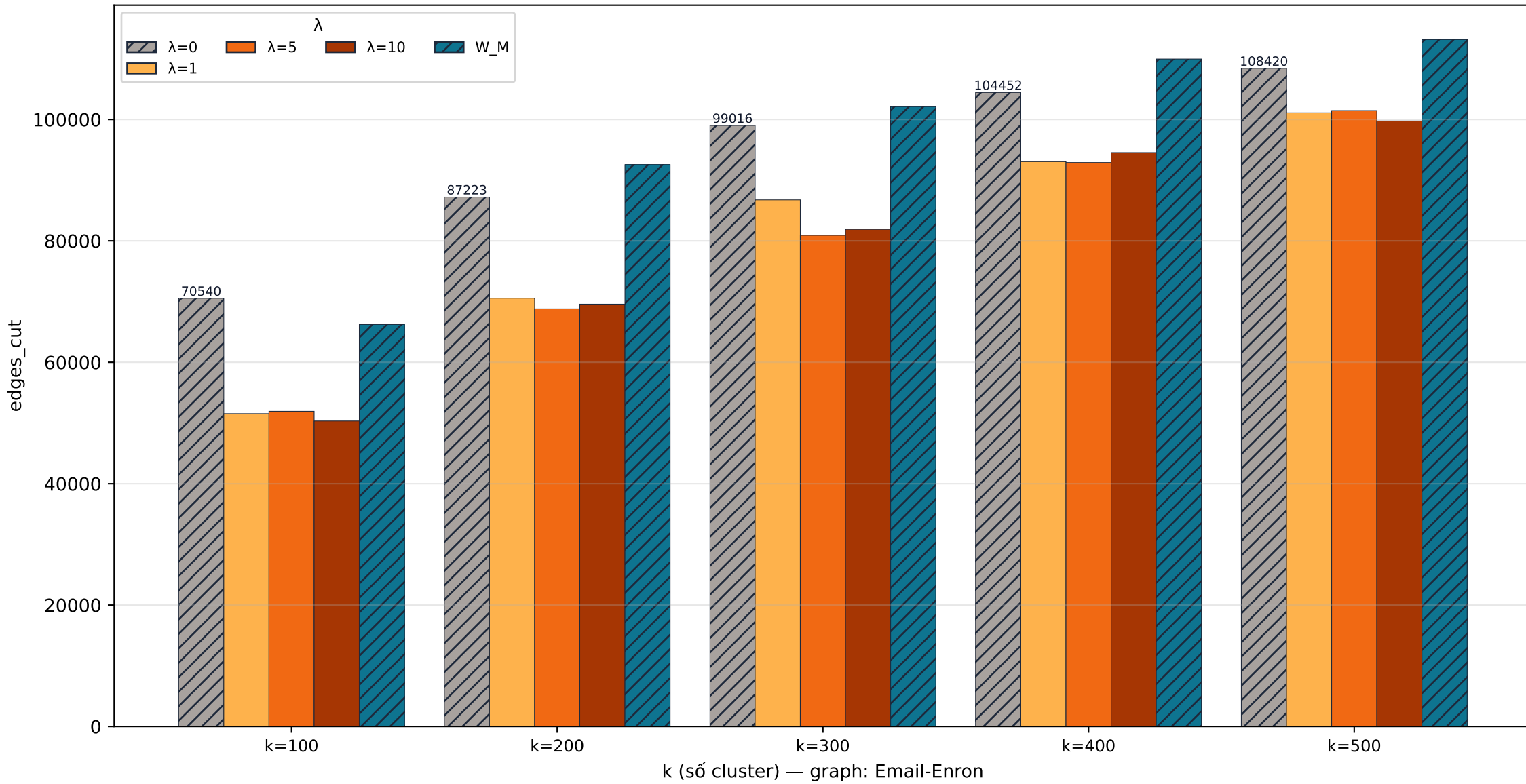
Email-Enron cut · edges_cut
