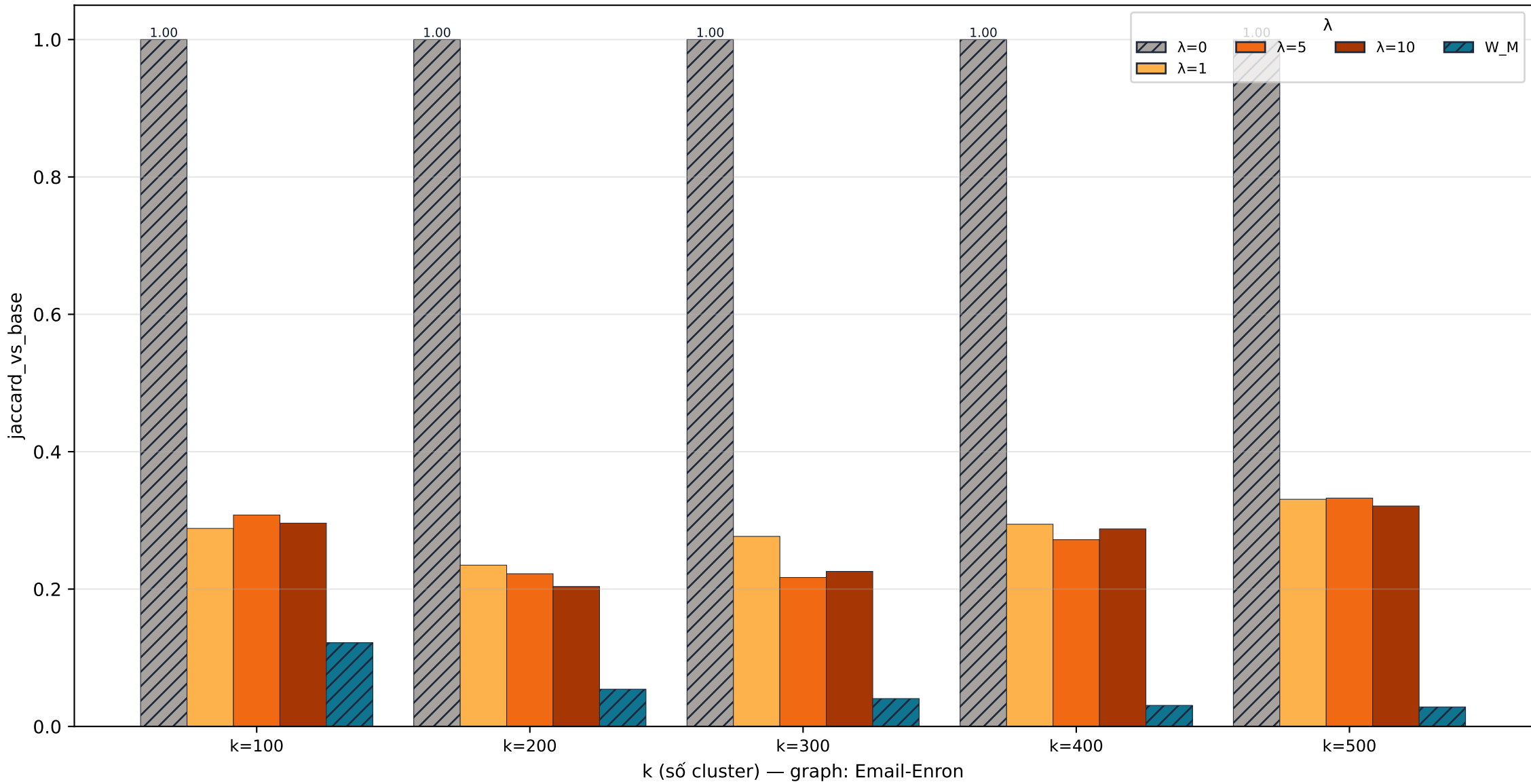
Email-Enron stability · jaccard_vs_base
