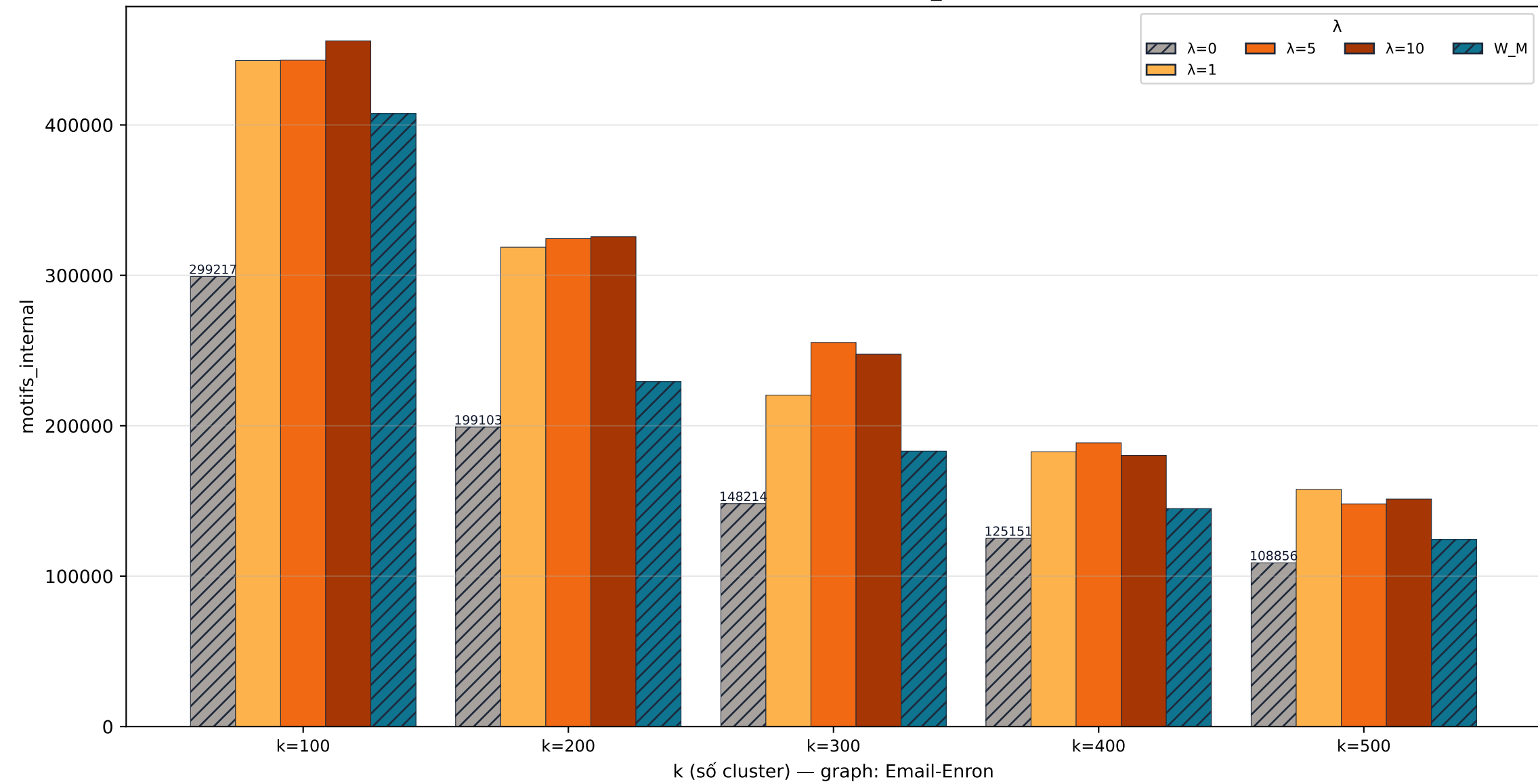
Email-Enron cut · motifs_internal
