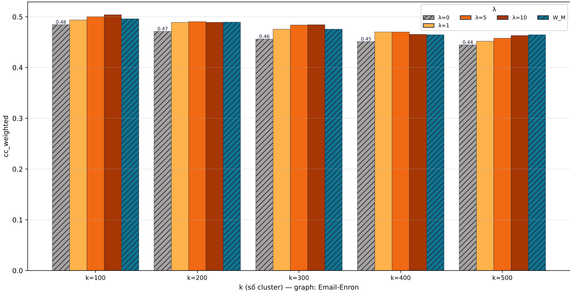
Email-Enron quality · cc_weighted
