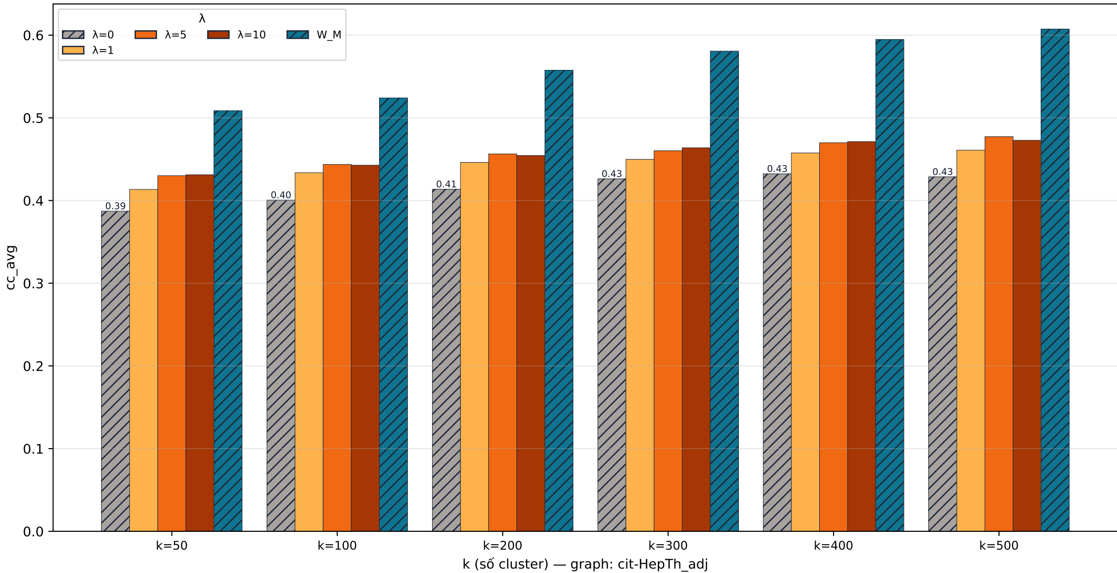
cit-HepTh_adj quality · cc_avg
