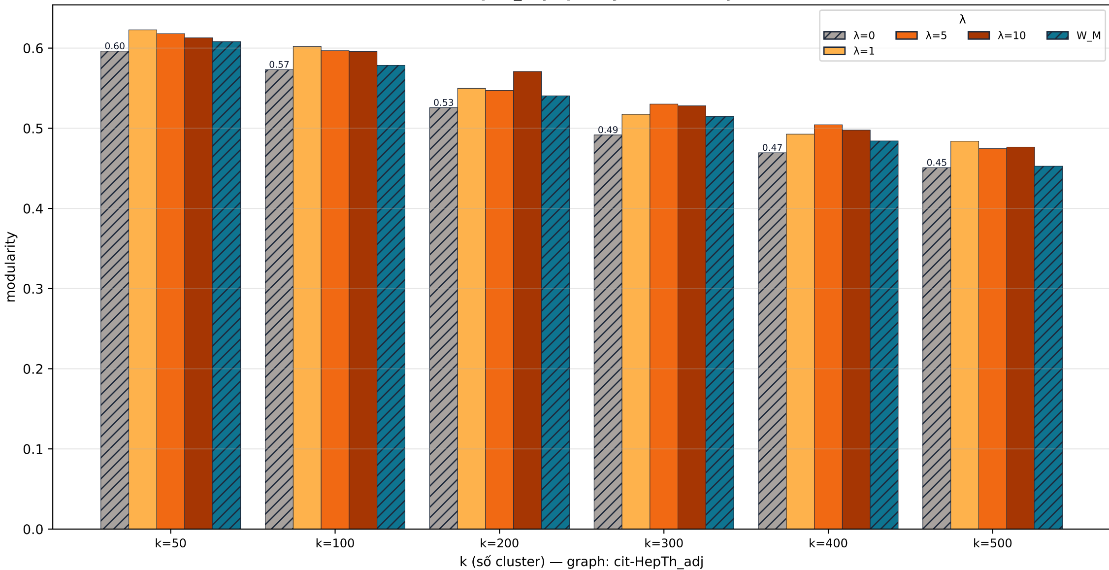
cit-HepTh_adj quality · modularity
