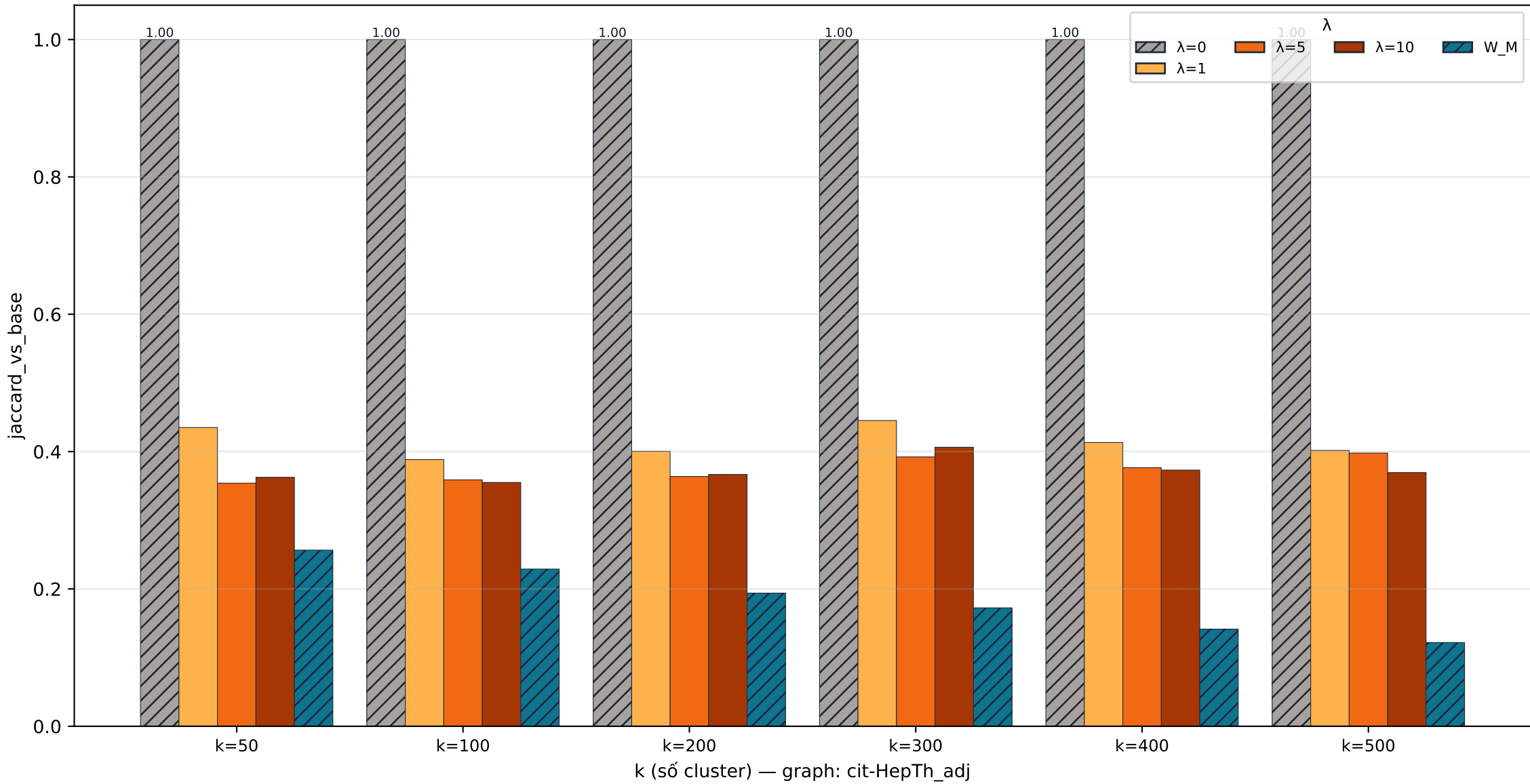
cit-HepTh_adj stability · jaccard_vs_base
