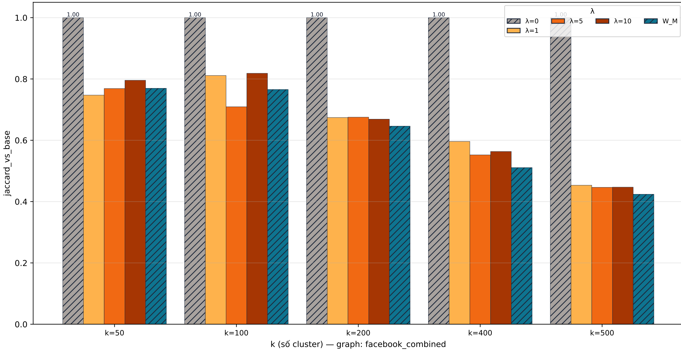
facebook_combined stability · jaccard_vs_base
