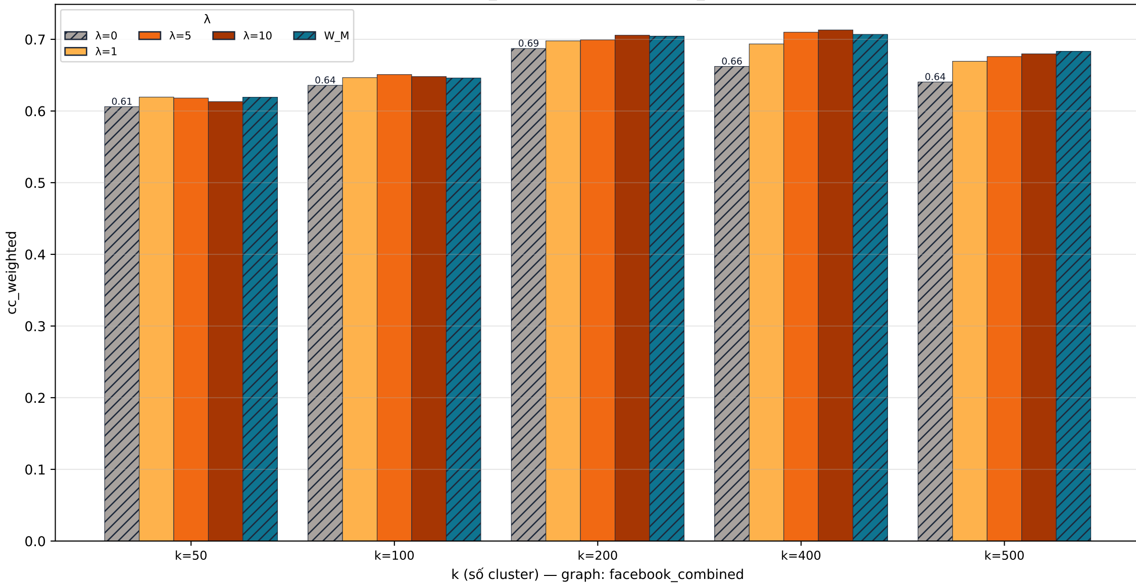
facebook_combined quality · cc_weighted
