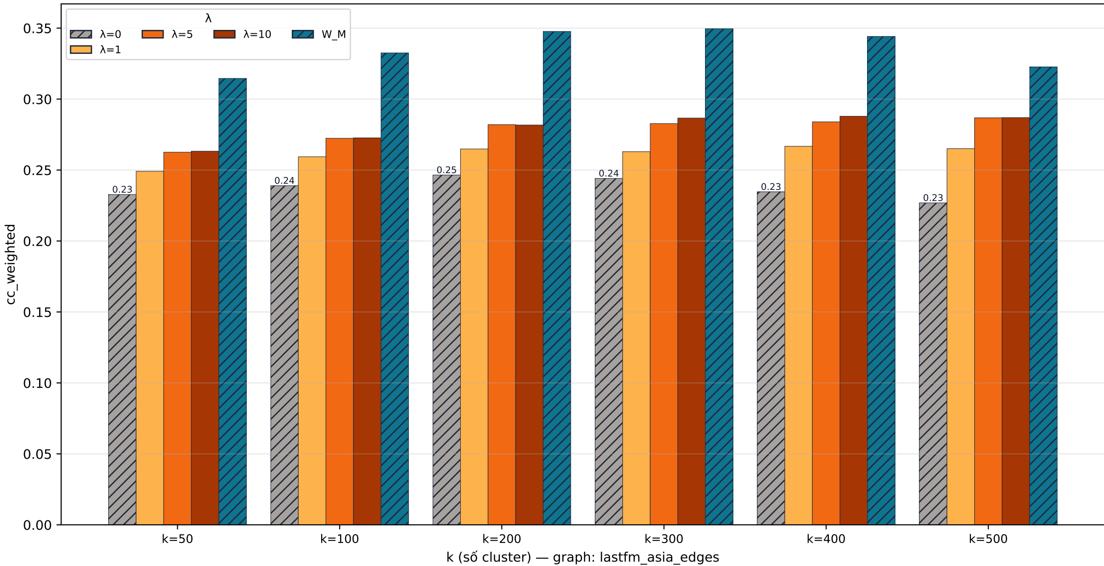
lastfm_asia_edges quality · cc_weighted
