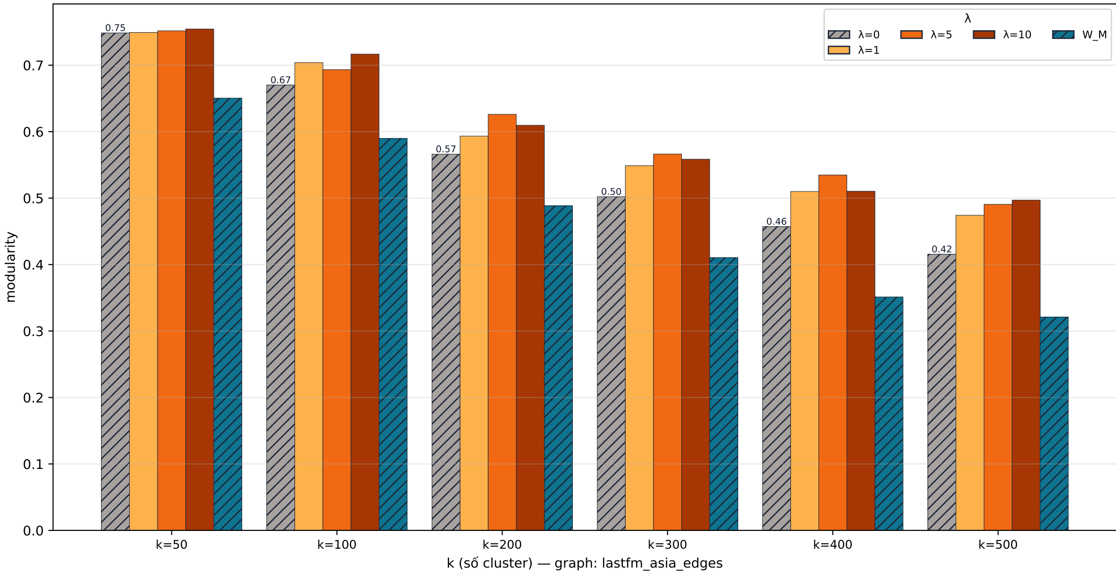
lastfm_asia_edges quality · modularity
