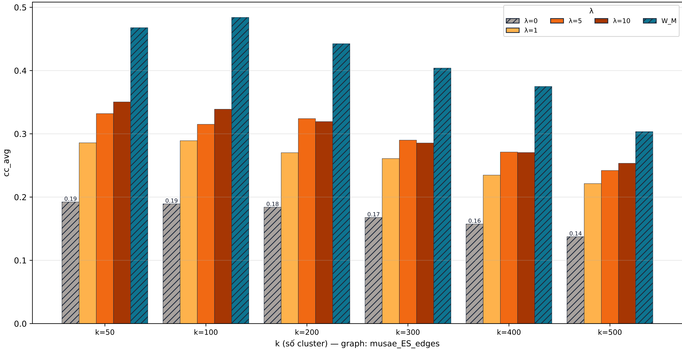
musae_ES_edges quality · cc_avg
