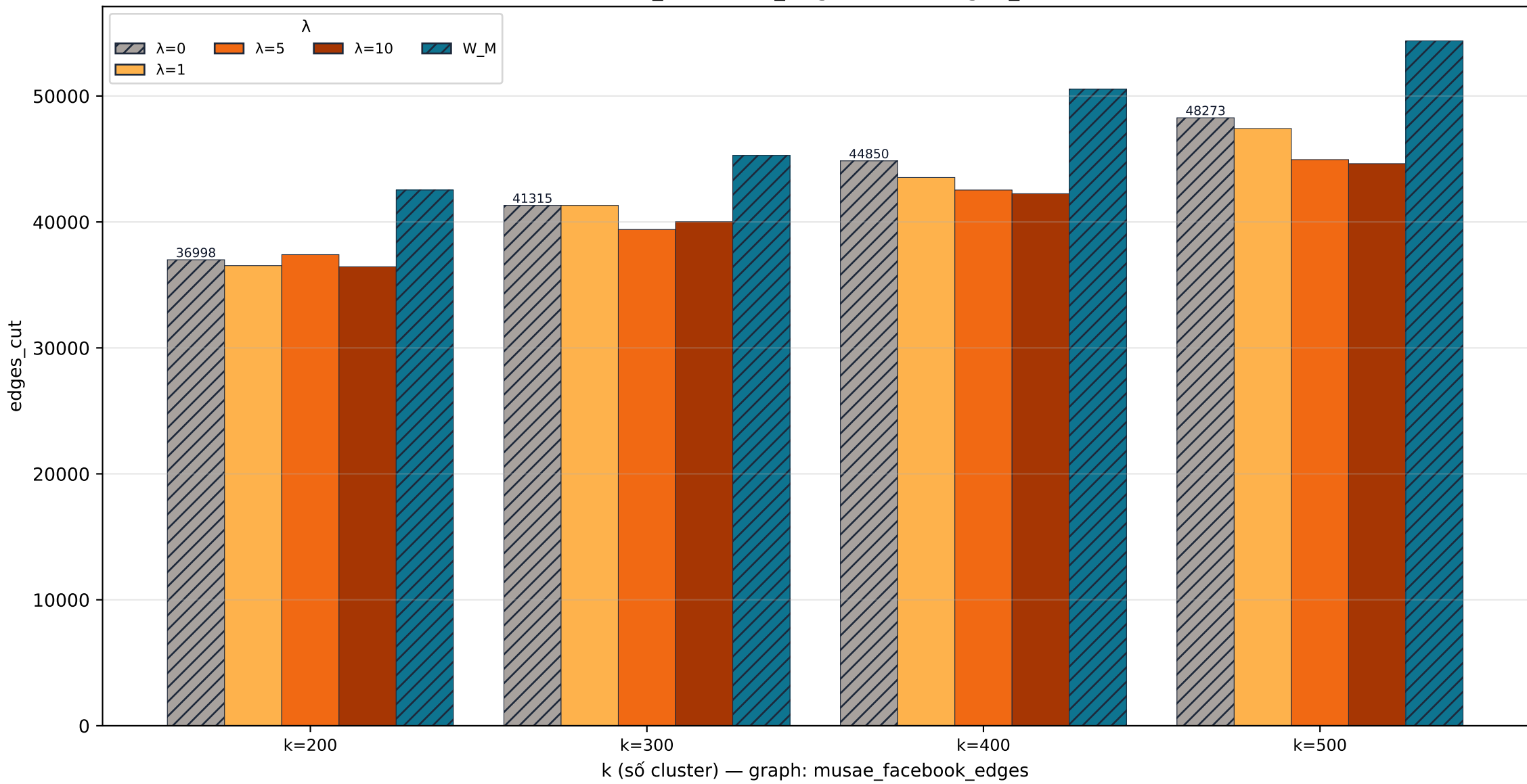
musae_facebook_edges cut · edges_cut
