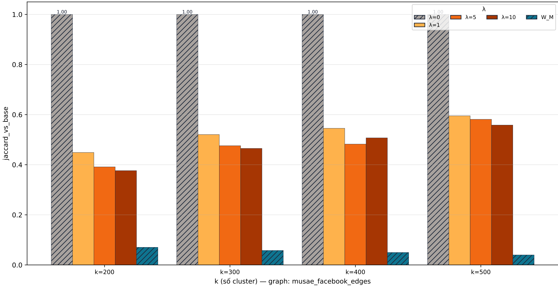
musae_facebook_edges stability · jaccard_vs_base
