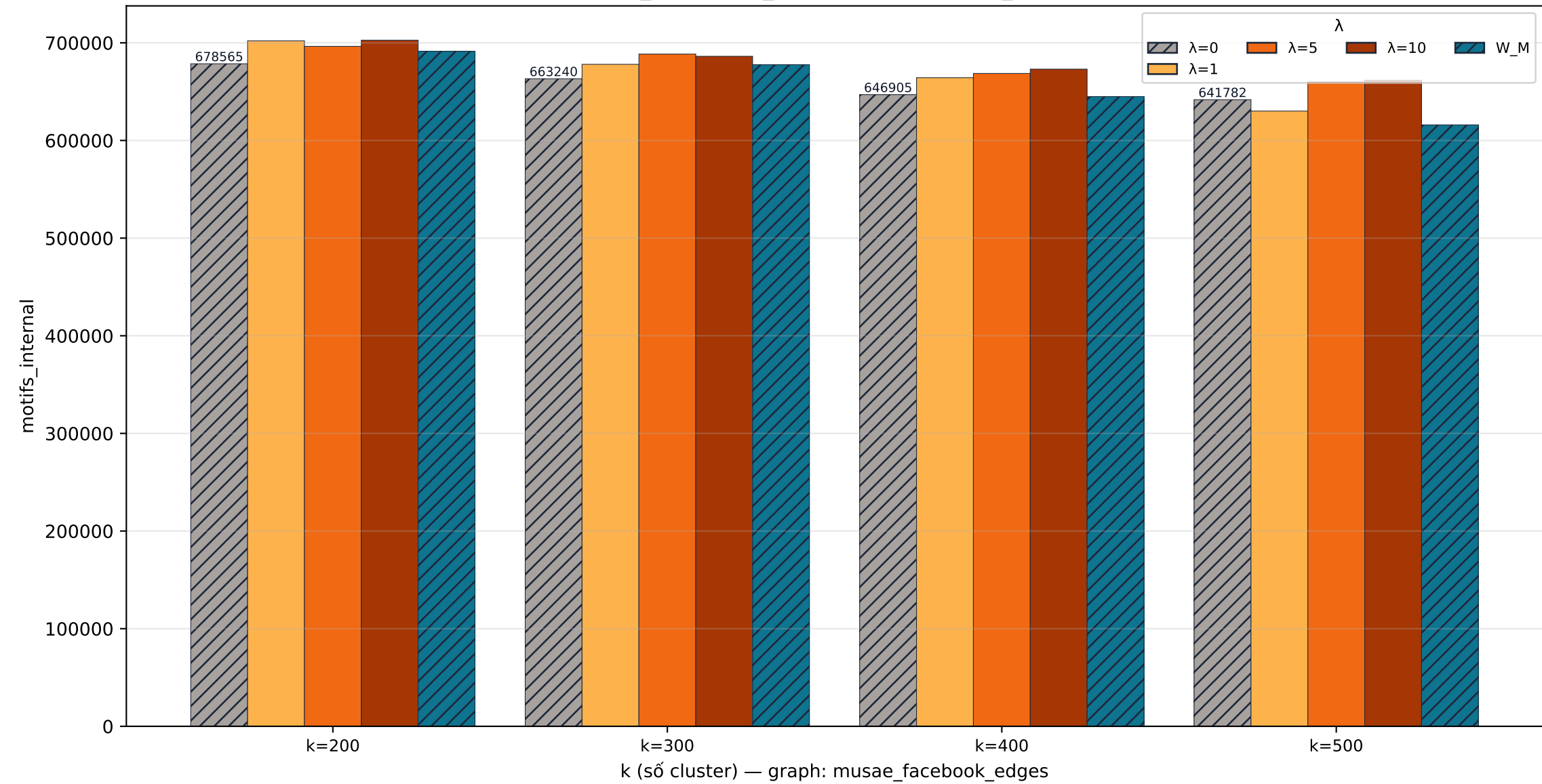
musae_facebook_edges cut · motifs_internal
