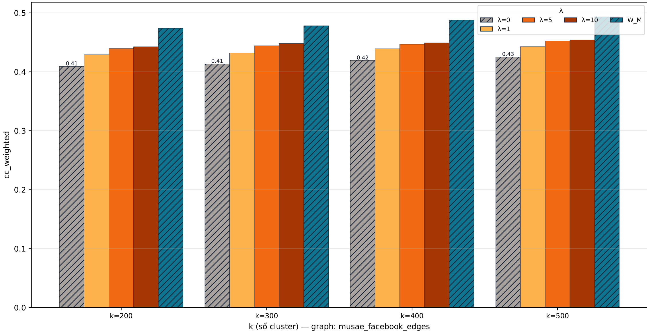
musae_facebook_edges quality · cc_weighted
