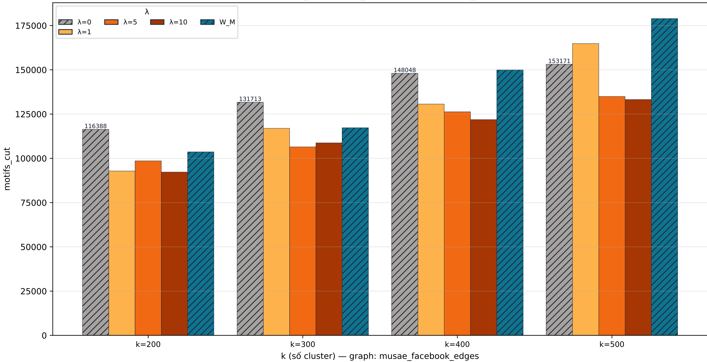
musae_facebook_edges cut · motifs_cut
