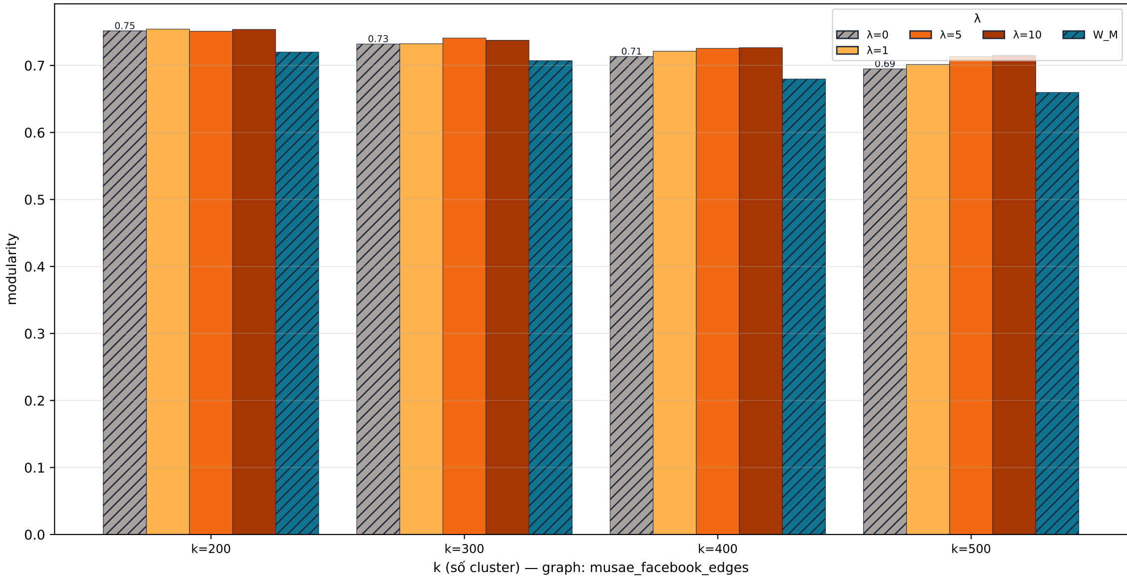
musae_facebook_edges quality · modularity
