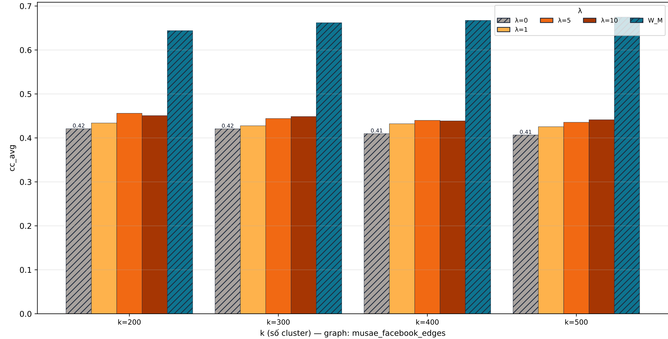
musae_facebook_edges quality · cc_avg
