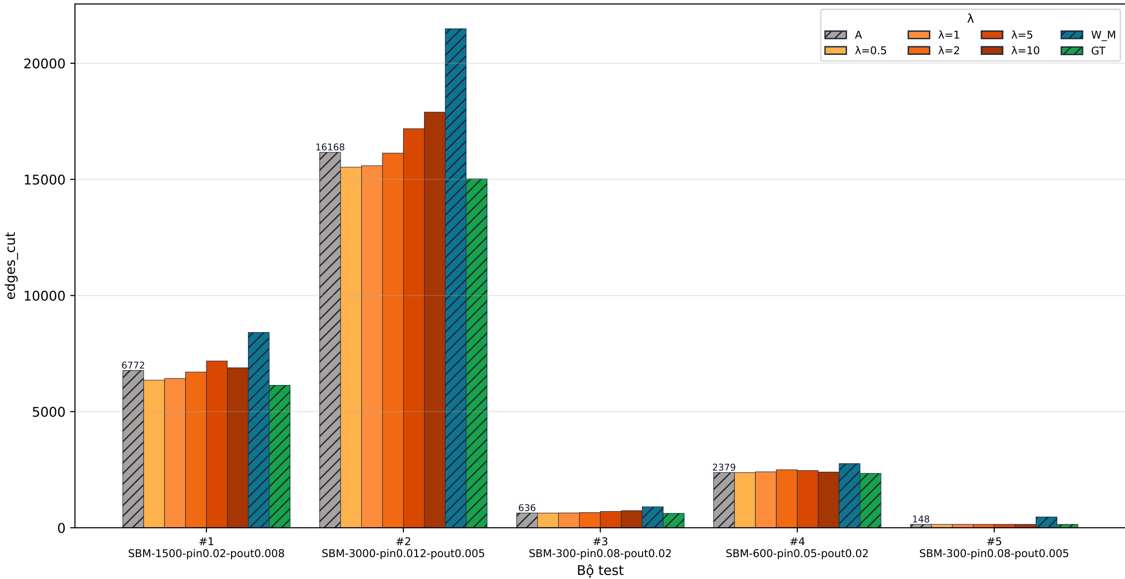
[SBM] cut · edges_cut
