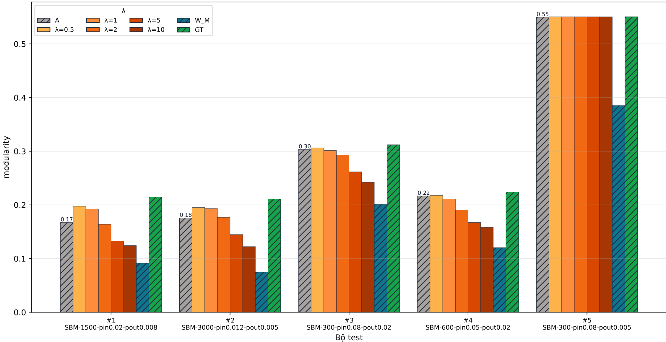
[SBM] quality · modularity
