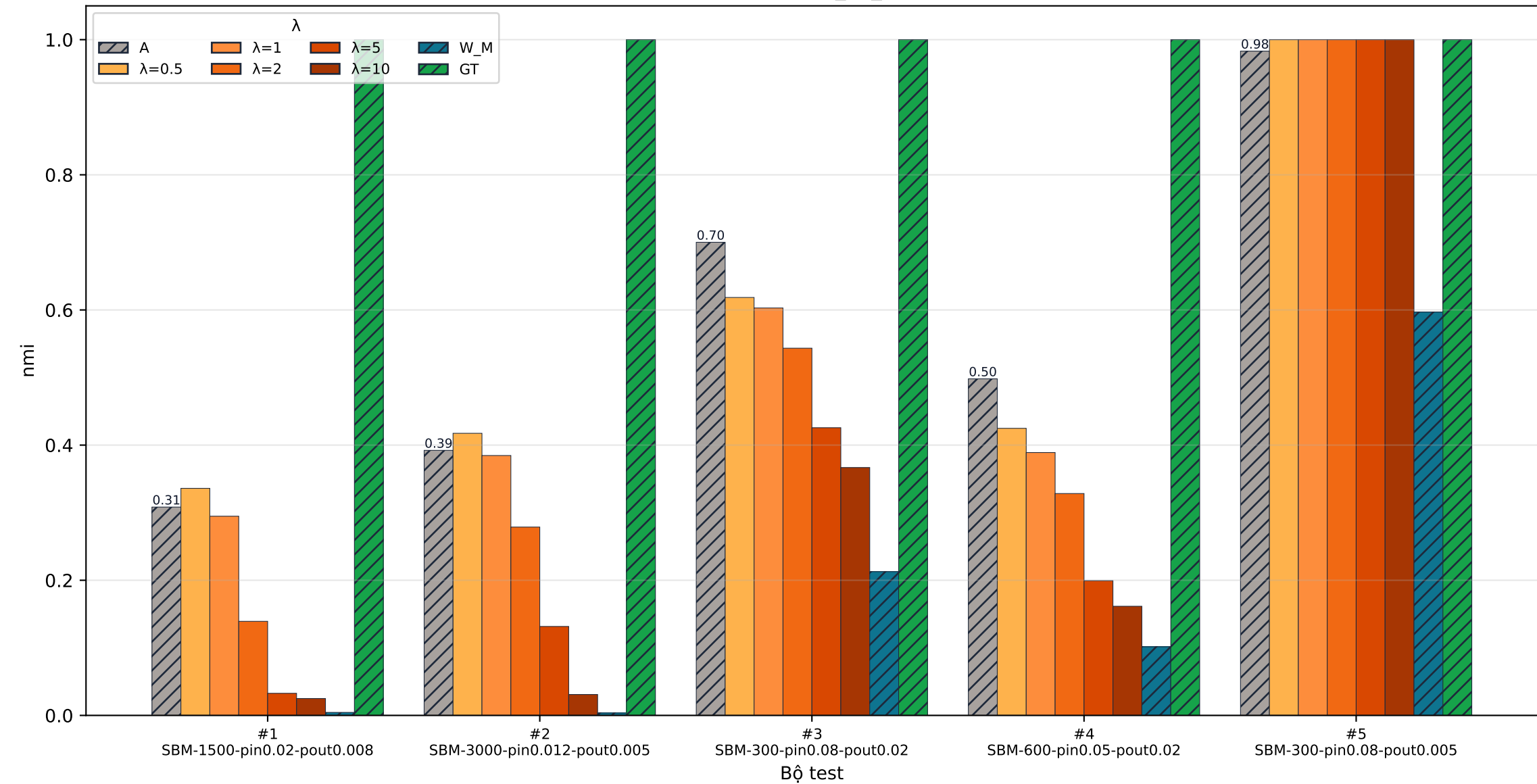
[SBM] compare_to_GT · nmi
