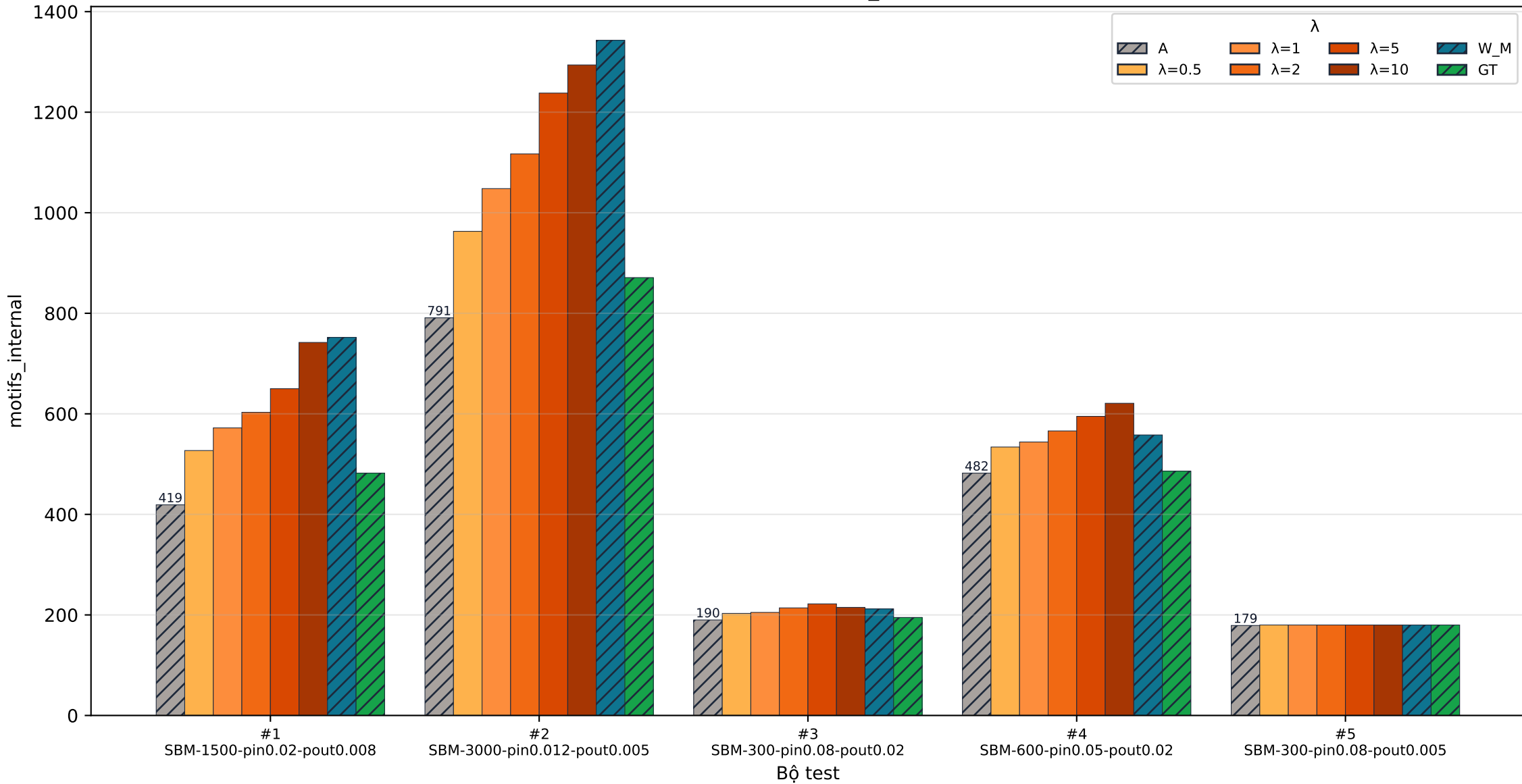
[SBM] cut · motifs_internal
