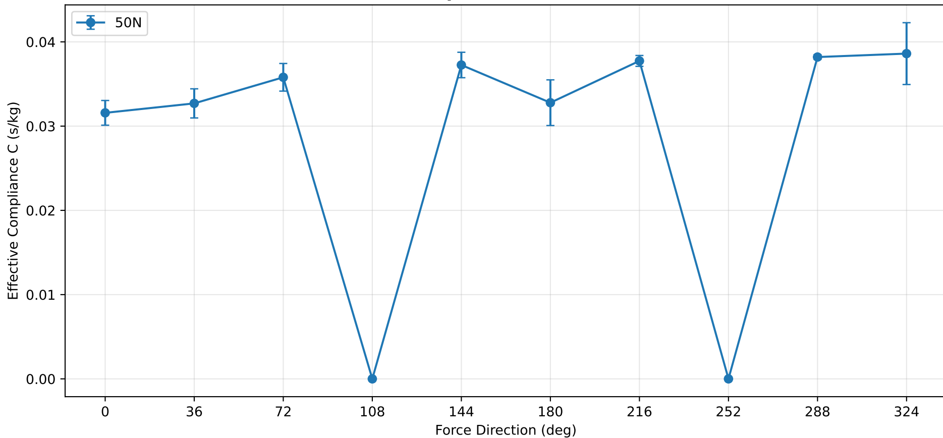
Effective Compliance vs Force Direction
