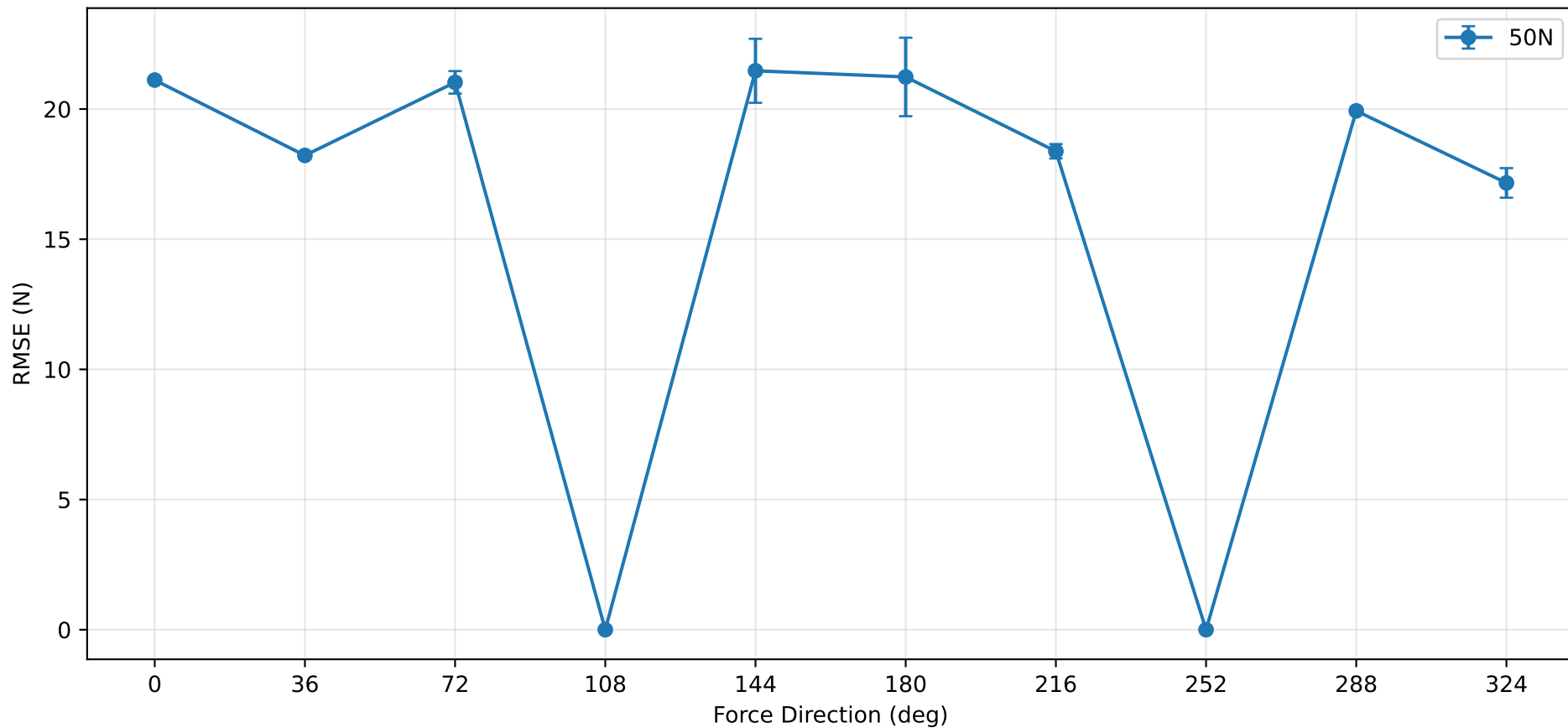
Force Estimator RMSE vs Direction
