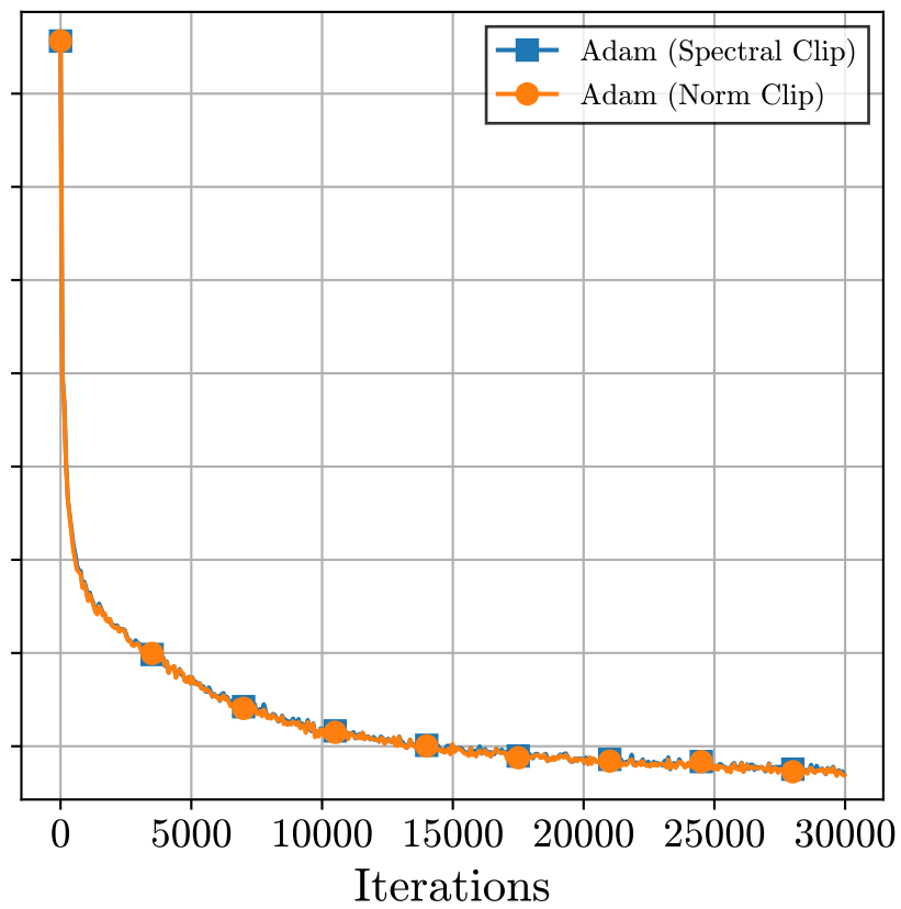
Adam
