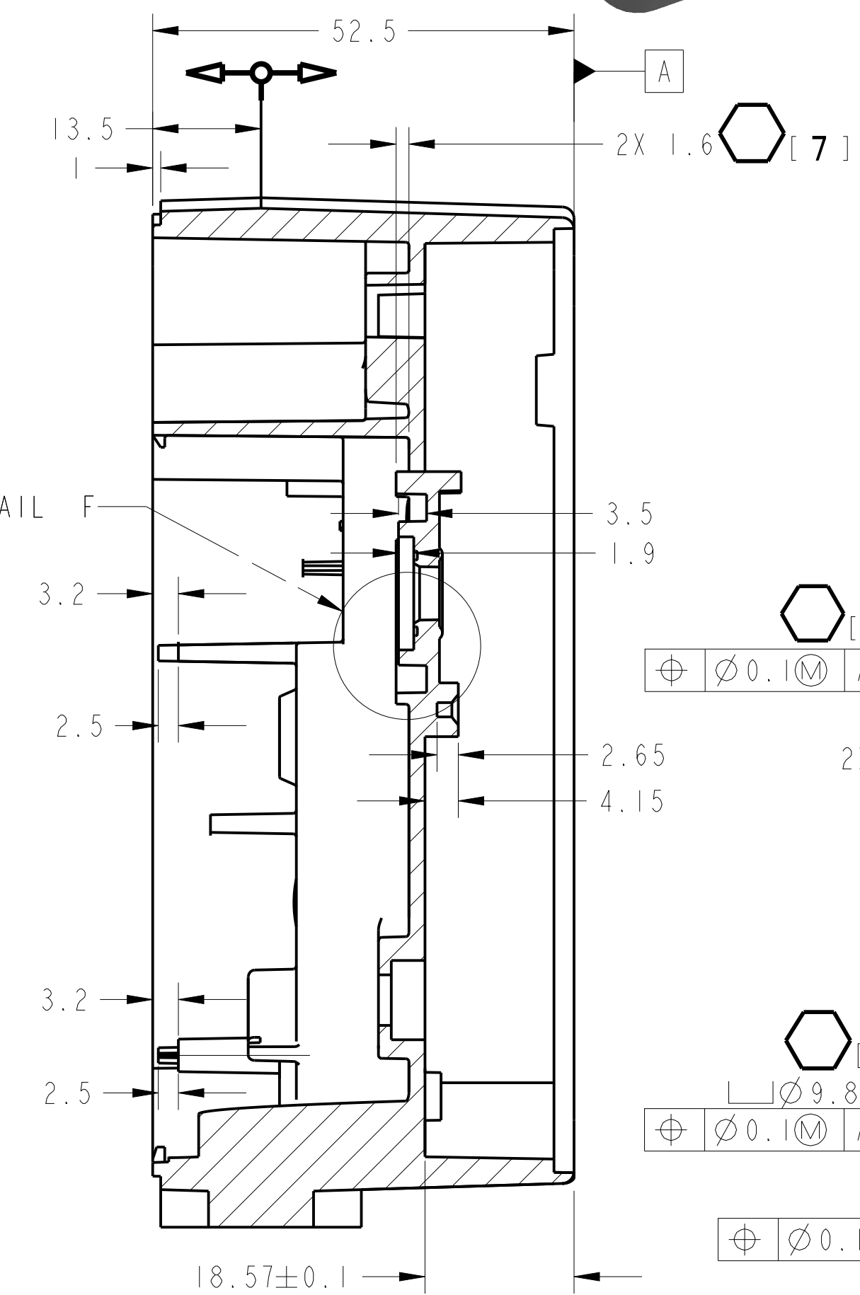
SECTION B-B
