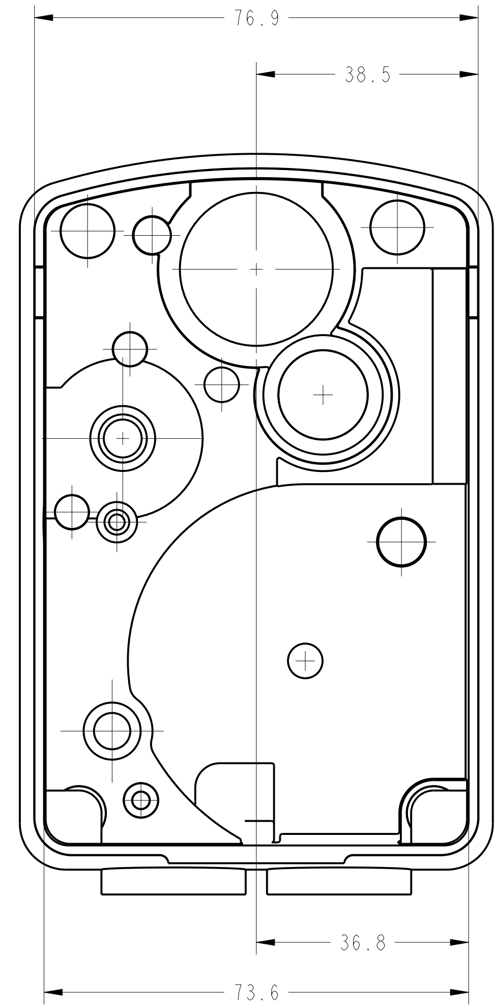
BACK VIEW
