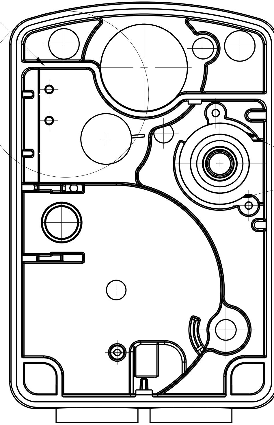
FRONT VIEW SHOWING 34-1770-22
