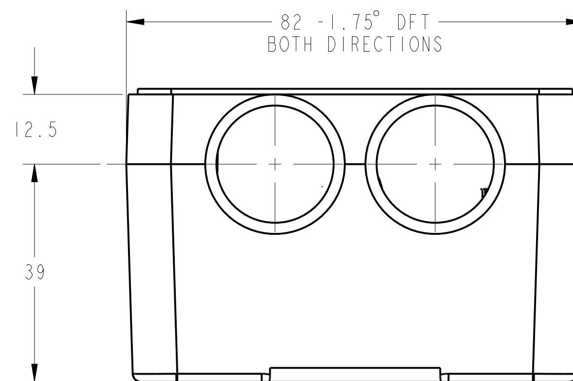
FRONT VIEW SHOWING 34-1770-22
