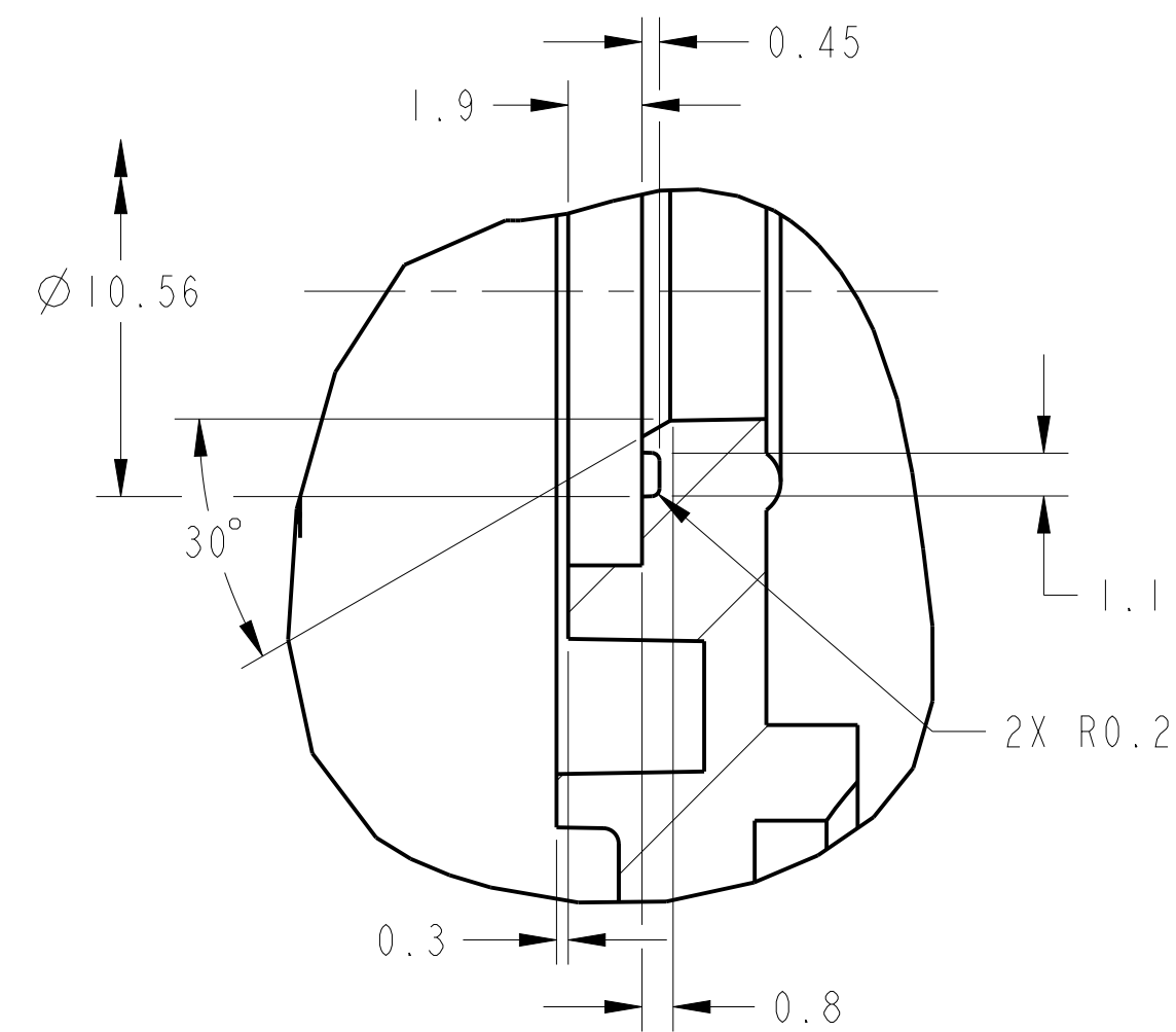
DETAIL F SCALE 5:1 FOR -6, -14 & -49 MODELS
