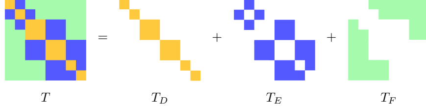
Figure 2: Illustration of the splitting of T : T_D is block diagonal with Toeplitz blocks, blocks in T_E are assumed to be well-approximated by low-rank matrices, and T_F is assumed to be small-norm due to weak interaction between elements.
