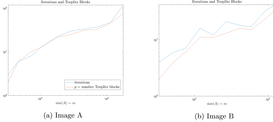
Figure 5: Iterations to convergence below a tolerance of \varepsilon = 10^{-7} for \alpha = 1.9 , plotted with the number of Toeplitz blocks across increasing matrix size m . Their approximate equality further supports the interpretation of 1 \times 1 blocks acting as additional boundaries imposed on the problem, requiring roughly one iteration for each outlier eigenvalue these boundaries cause.
