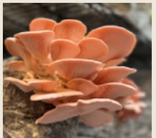
Pink Oyster
