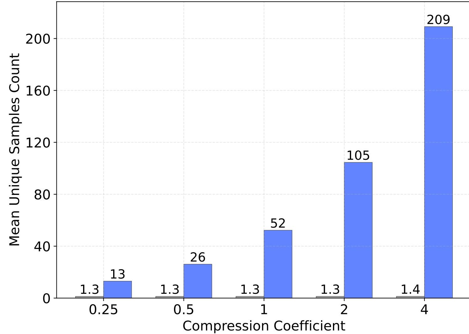
Unique Samples Comparison Higher is better
