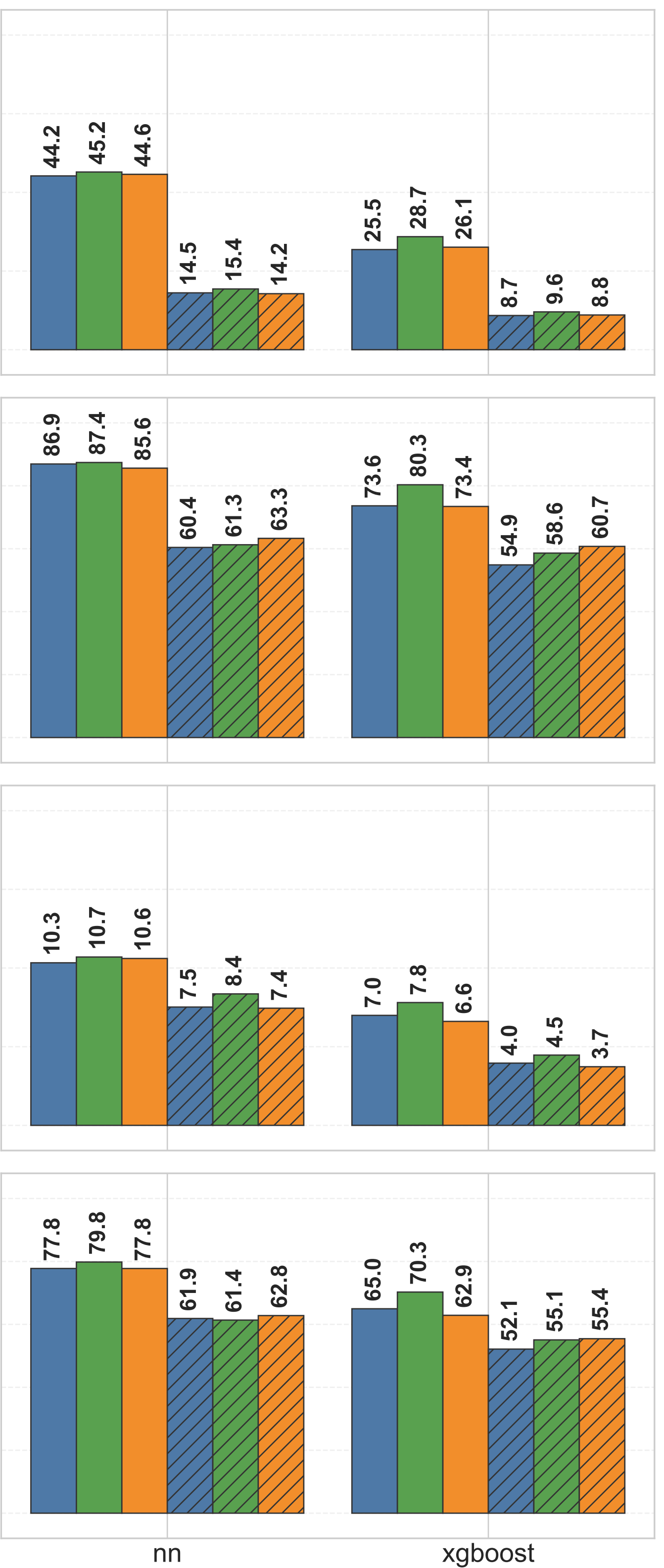
SHAP-IQ (Kernel)
