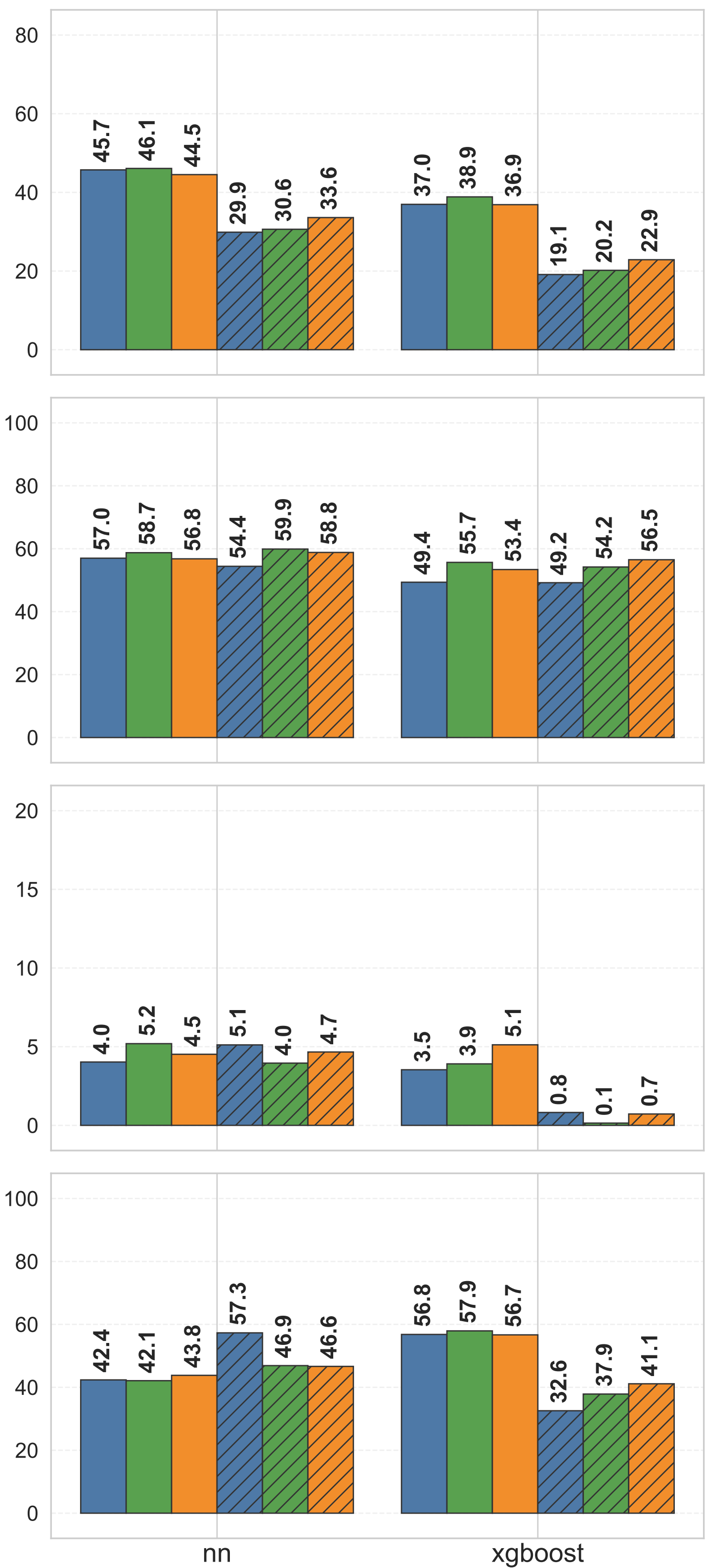
SAGE (Permutation)
