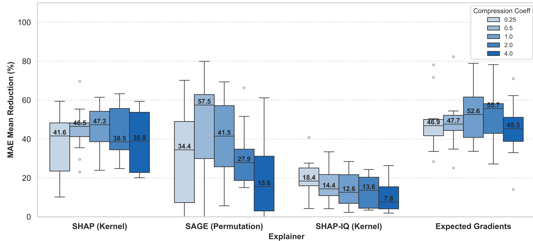
Model: NN | Task: Classification
