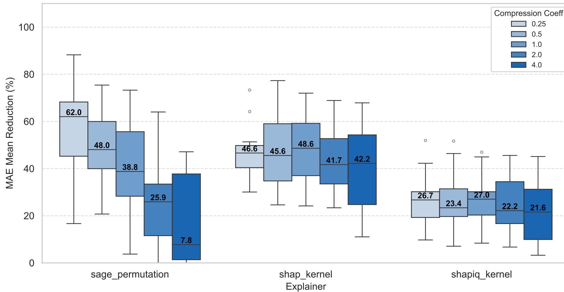
Model: XGBOOST | Task: Regression
