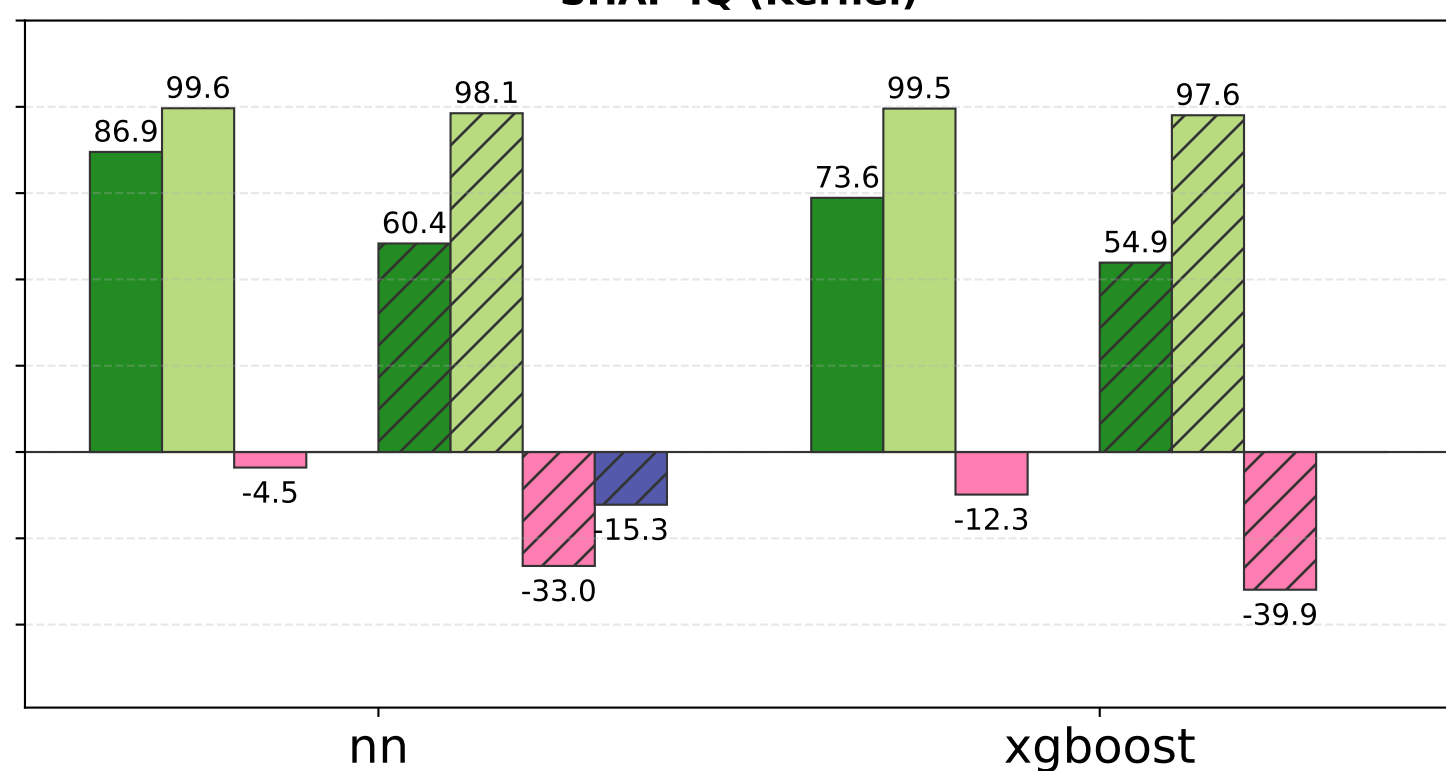
SHAP-IQ (Kernel)
