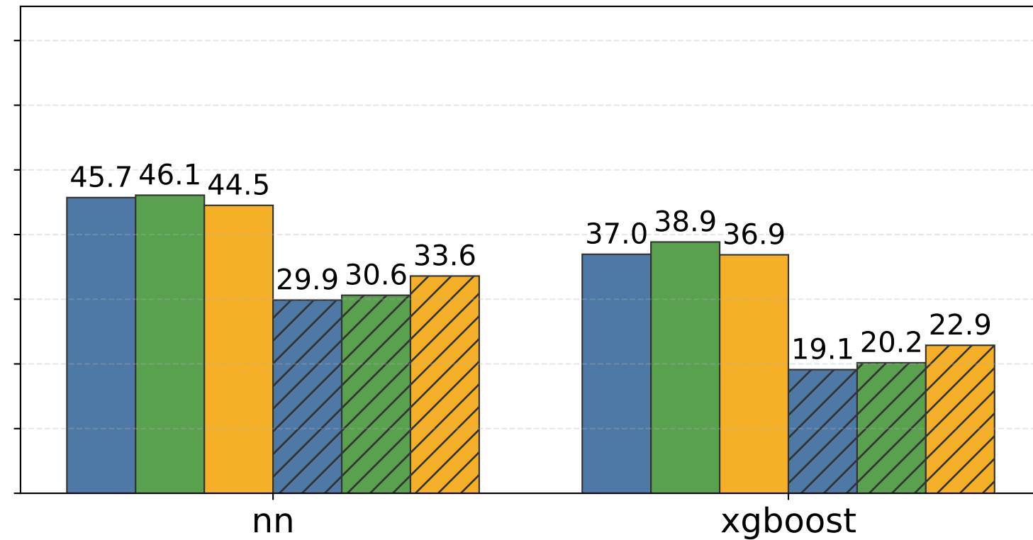
SHAP-IQ (Kernel)
