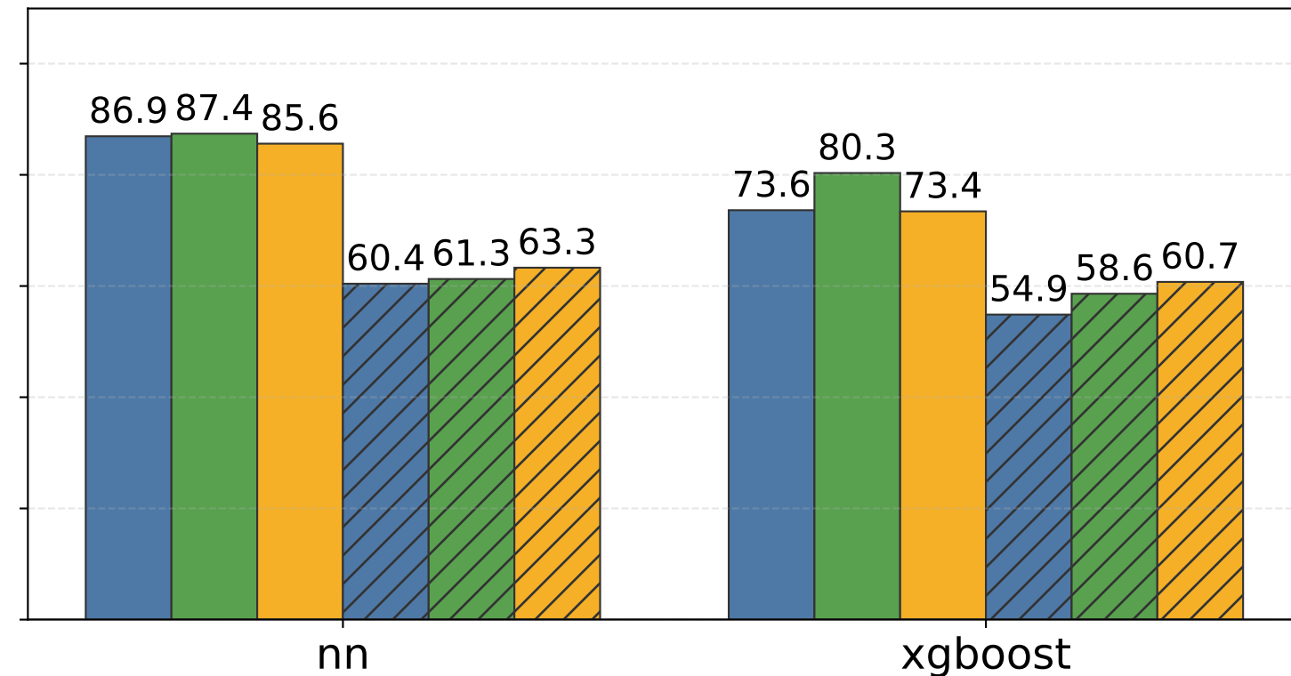
SHAP-IQ (Kernel)
