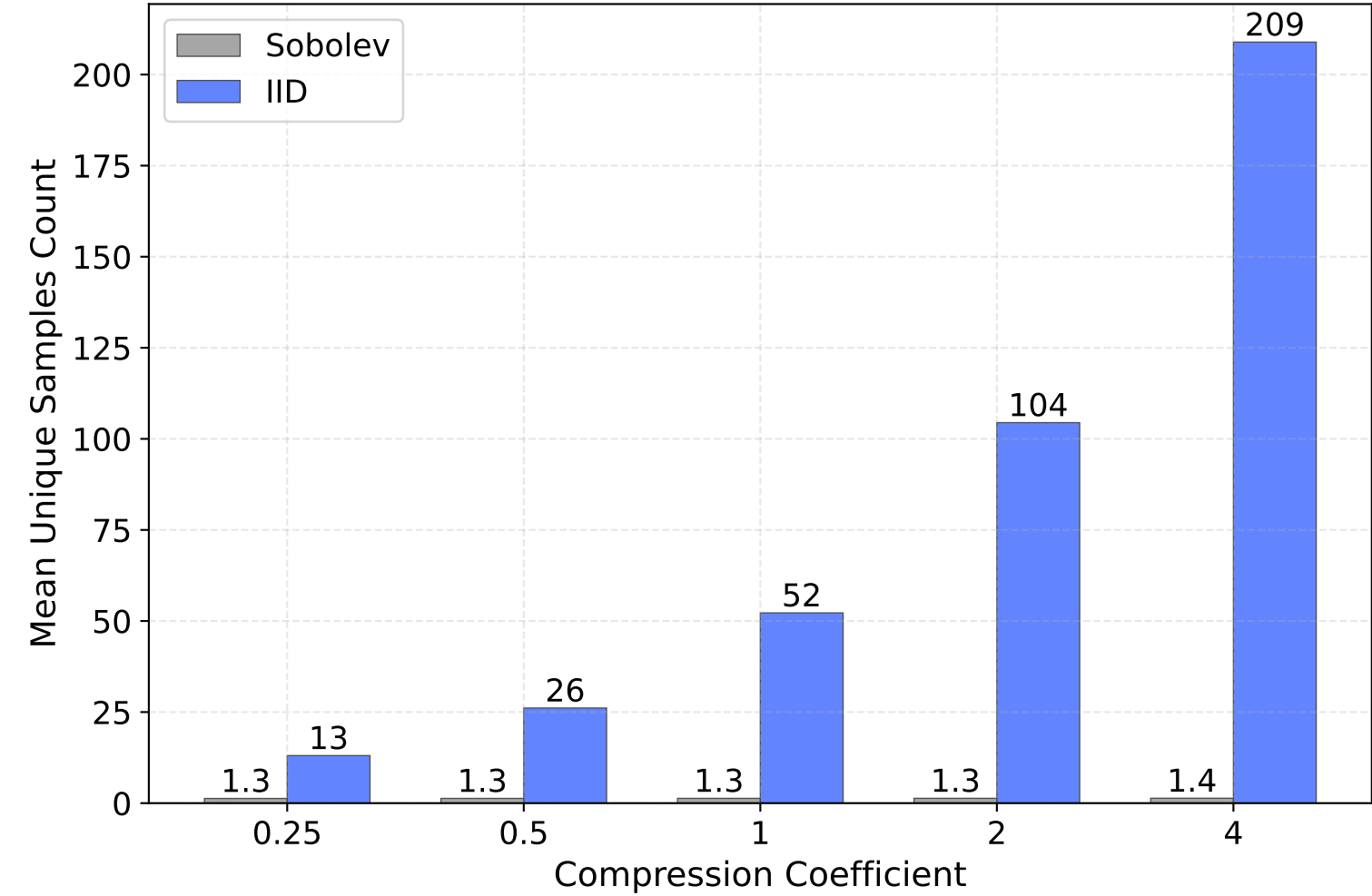
Unique Samples Comparison Higher is better
