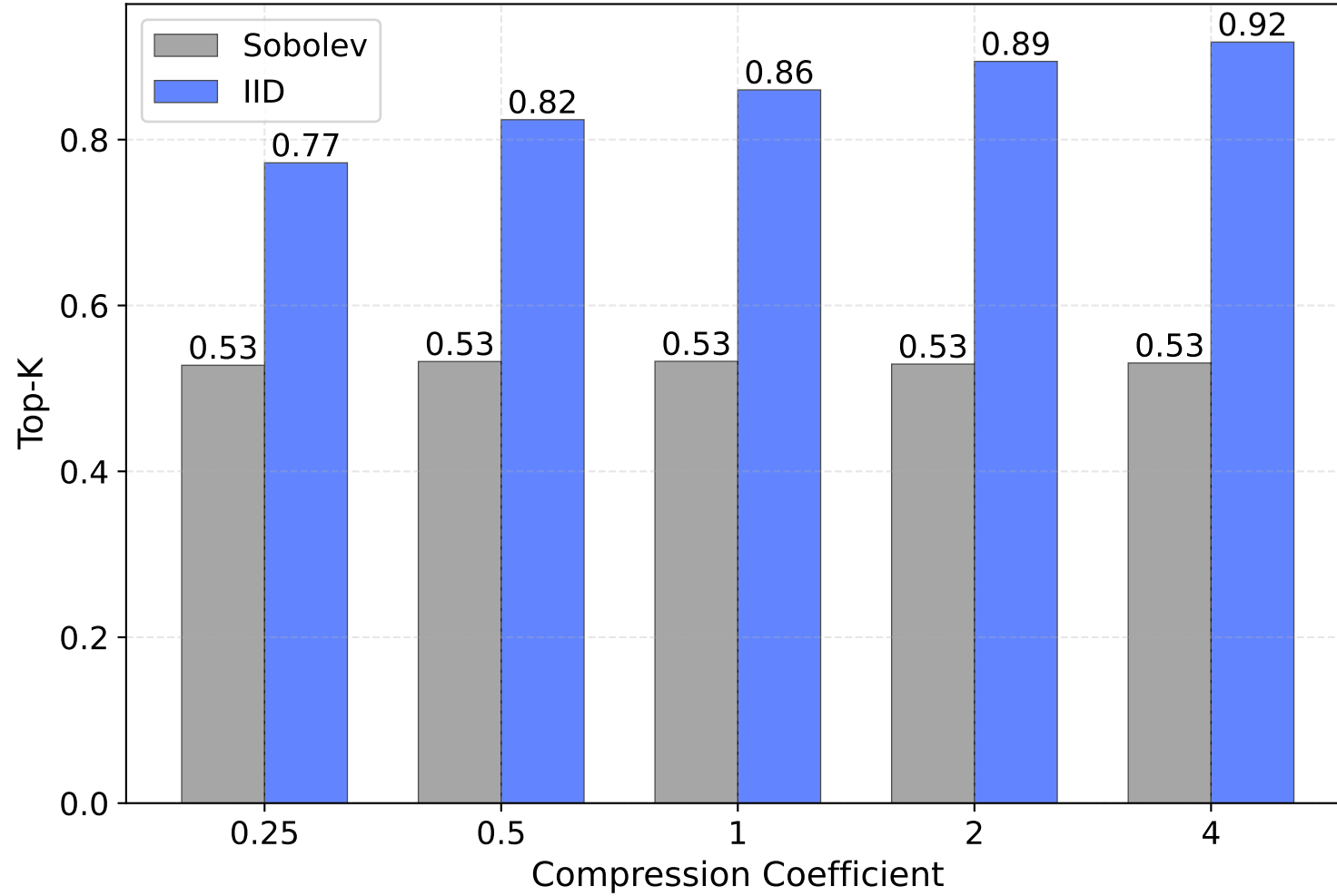
Top-K Comparison Higher is better
