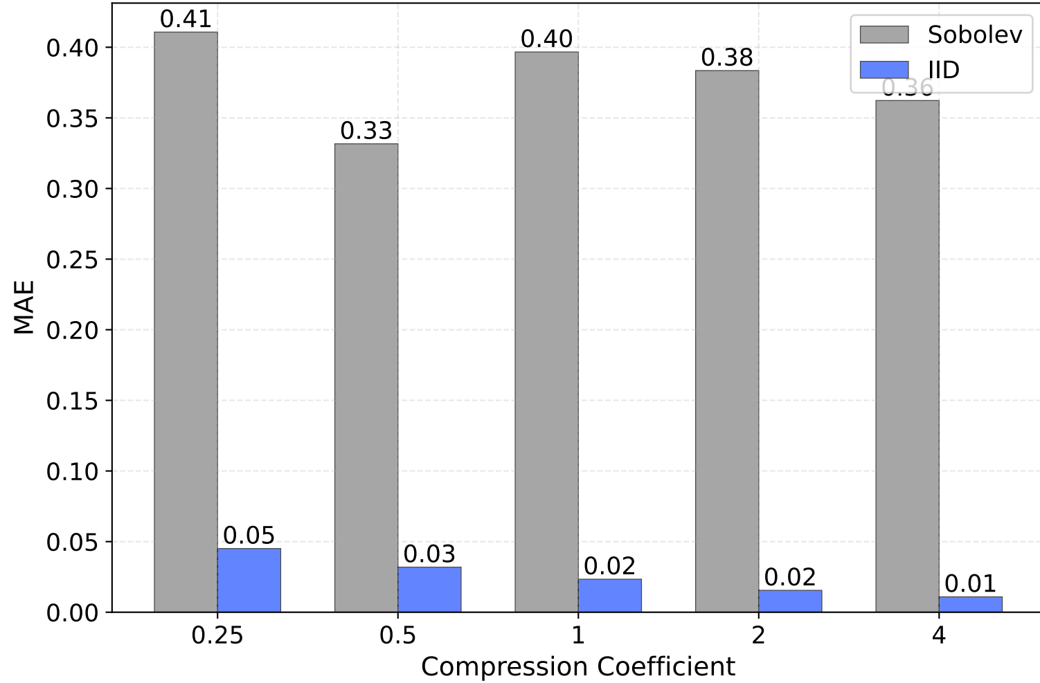
MAE Comparison Lower is better
