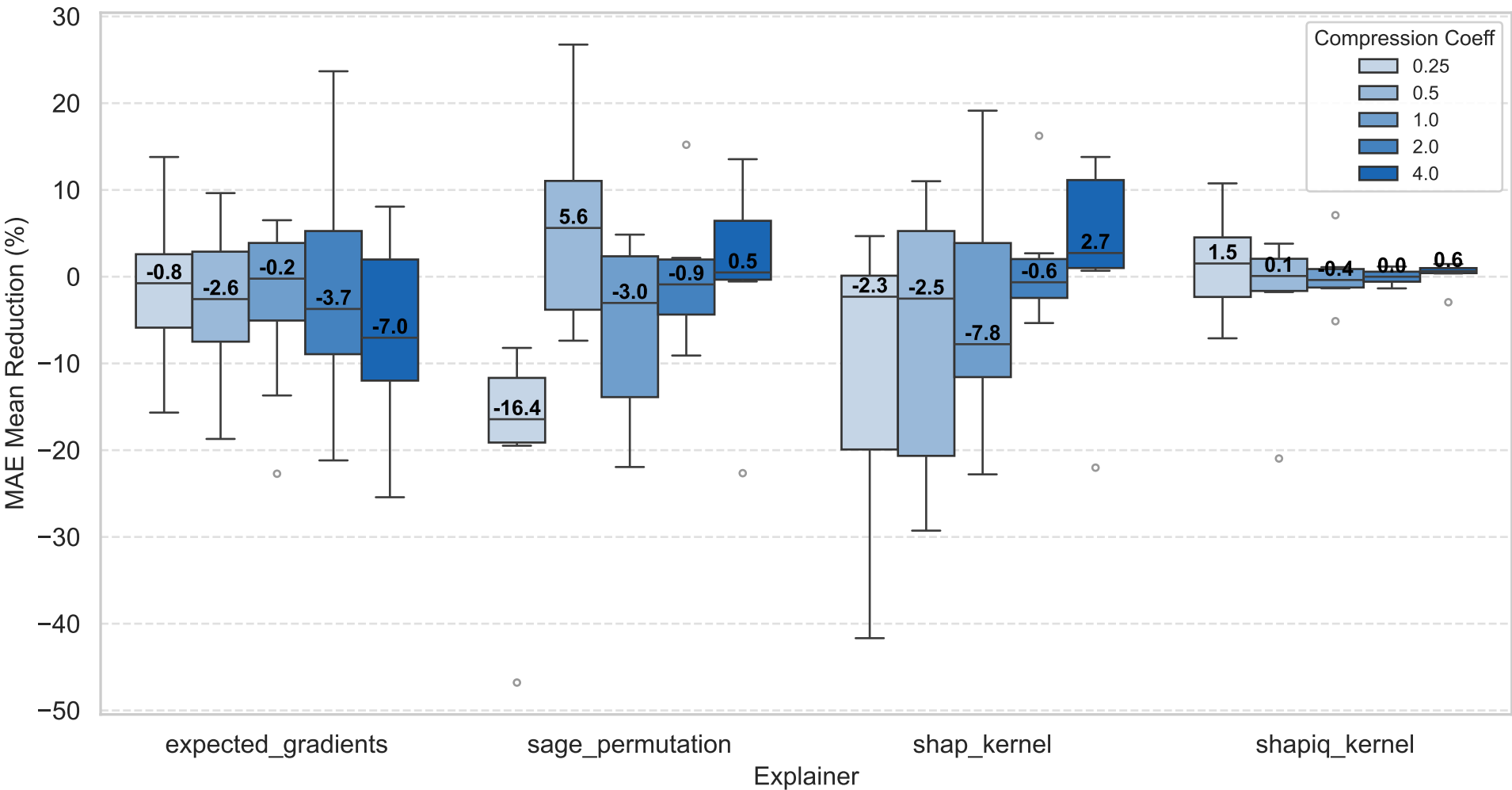
Model: XGBOOST | Task: Classification
