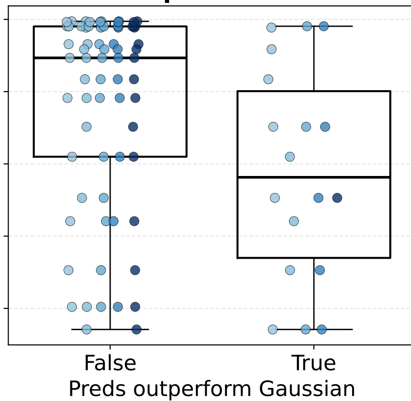
Top-K mean
