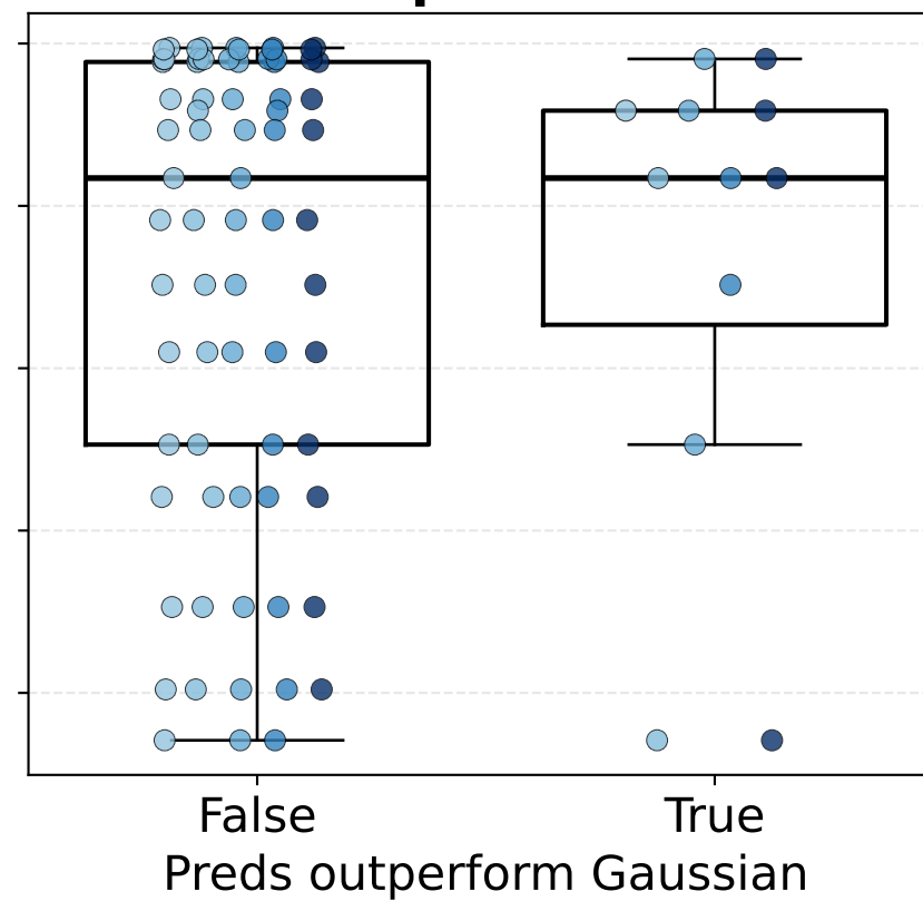
Top-K std
