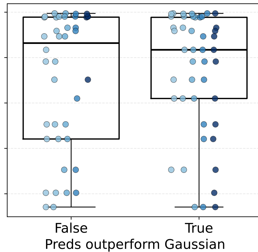
MAE std
