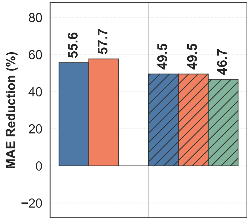
Expected Gradients
