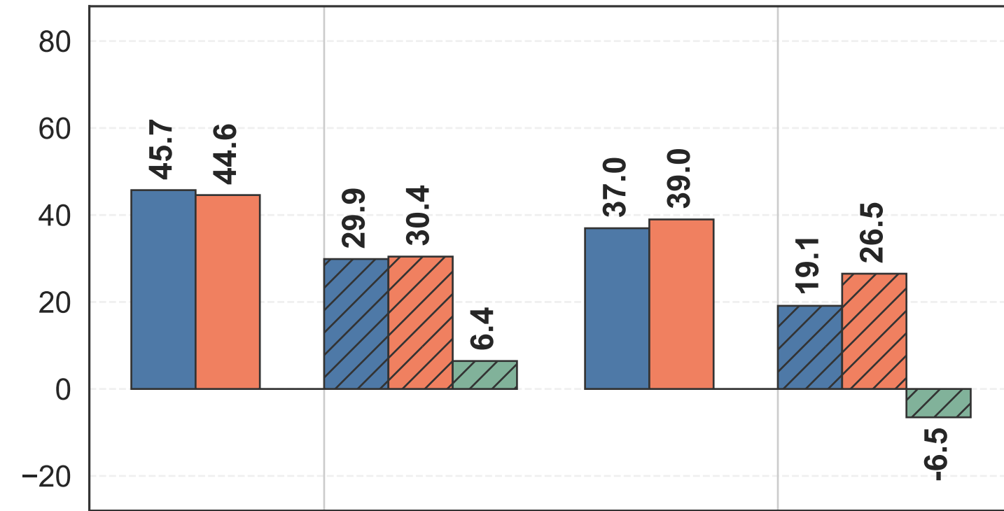
SAGE (Permutation)
