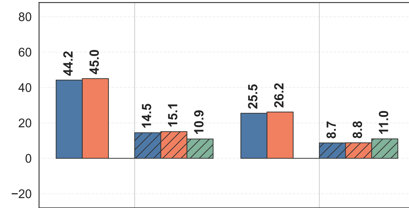
SHAP-IQ (Kernel)
