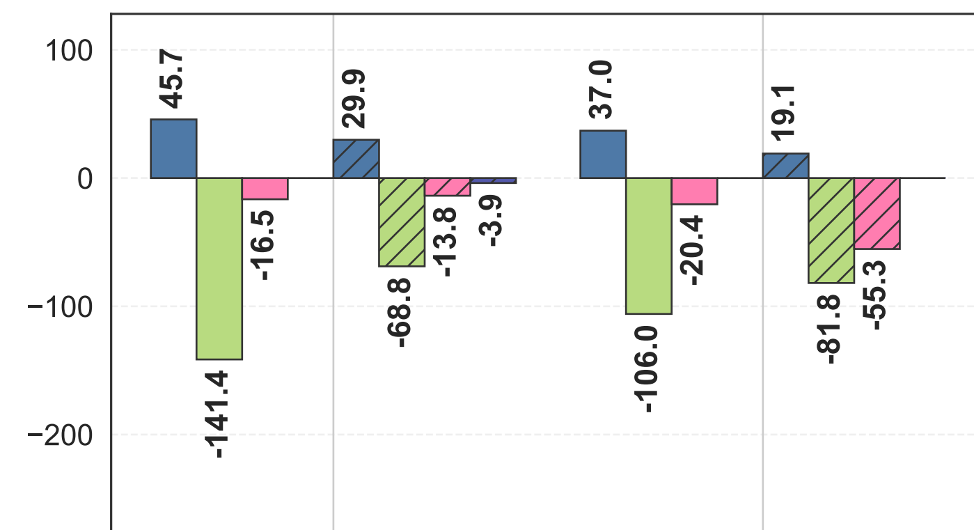
SAGE (Permutation)
