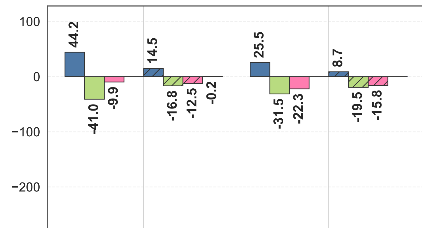
SHAP-IQ (Kernel)
