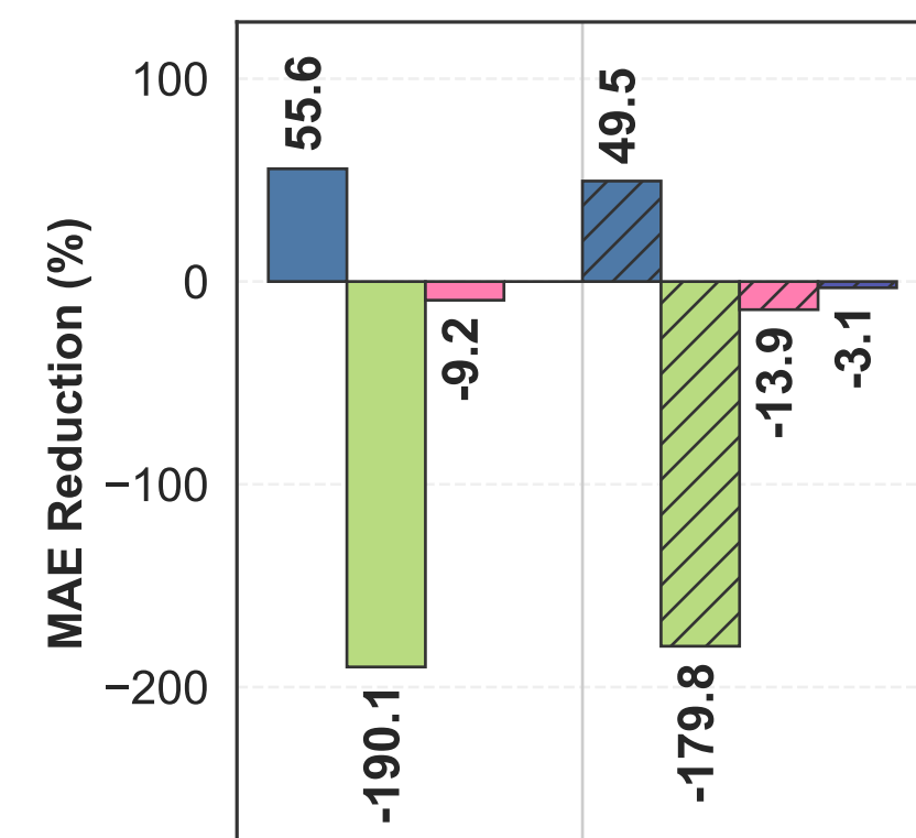
Expected Gradients
